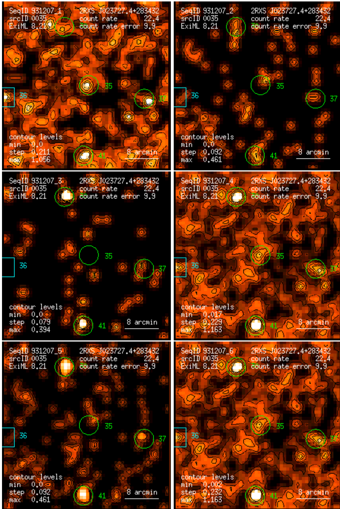
Figure 35: RASS 931207: detection 0035: band rate images, Gaussian filter: (1) PSPC channels 11 – 41, (2) 52 – 90, (3) 91 – 201, (4) 11 – 235, (5) 52 – 201, (6) 11 – 201. Broad band rates in counts/ks. Band rate contour levels in counts/ks/arcmin 2 .
