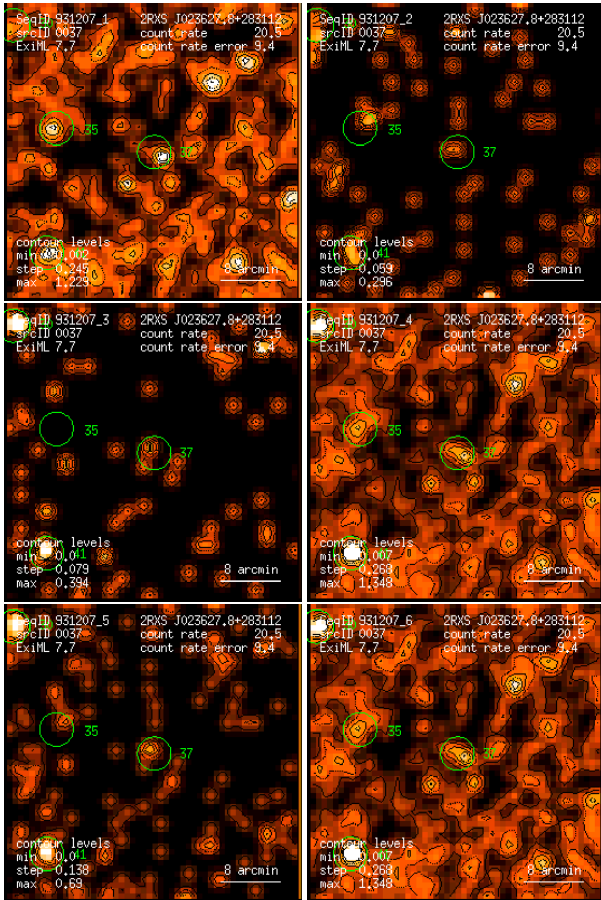
Figure 37: RASS 931207: detection 0037: band rate images, Gaussian filter: (1) PSPC channels 11 – 41, (2) 52 – 90, (3) 91 – 201, (4) 11 – 235, (5) 52 – 201, (6) 11 – 201. Broad band rates in counts/ks. Band rate contour levels in counts/ks/arcmin 2 .
