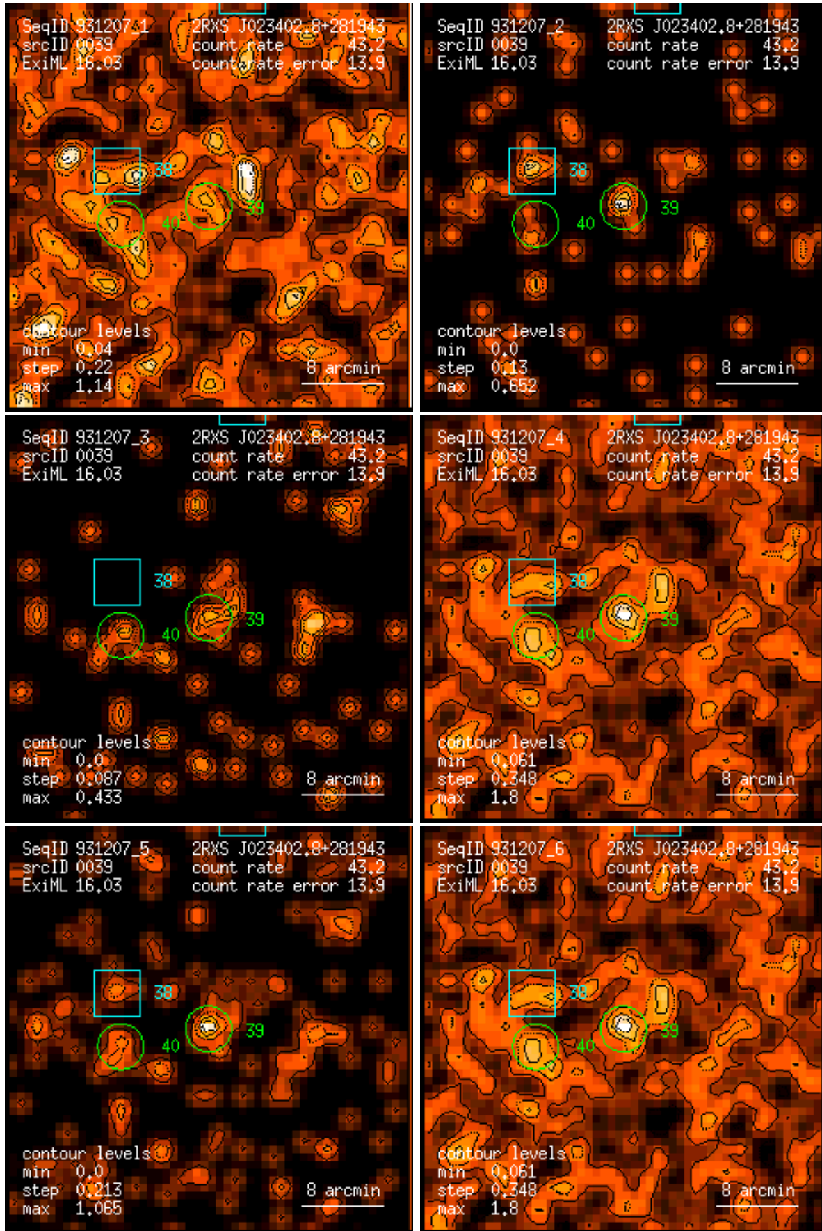
Figure 39: RASS 931207: detection 0039: band rate images, Gaussian filter: (1) PSPC channels 11 – 41, (2) 52 – 90, (3) 91 – 201, (4) 11 – 235, (5) 52 – 201, (6) 11 – 201. Broad band rates in counts/ks. Band rate contour levels in counts/ks/arcmin 2 .
