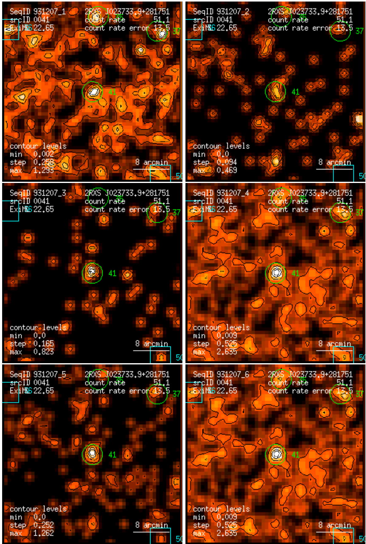
Figure 41: RASS 931207: detection 0041: band rate images, Gaussian filter: (1) PSPC channels 11 – 41, (2) 52 – 90, (3) 91 – 201, (4) 11 – 235, (5) 52 – 201, (6) 11 – 201. Broad band rates in counts/ks. Band rate contour levels in counts/ks/arcmin 2 .
