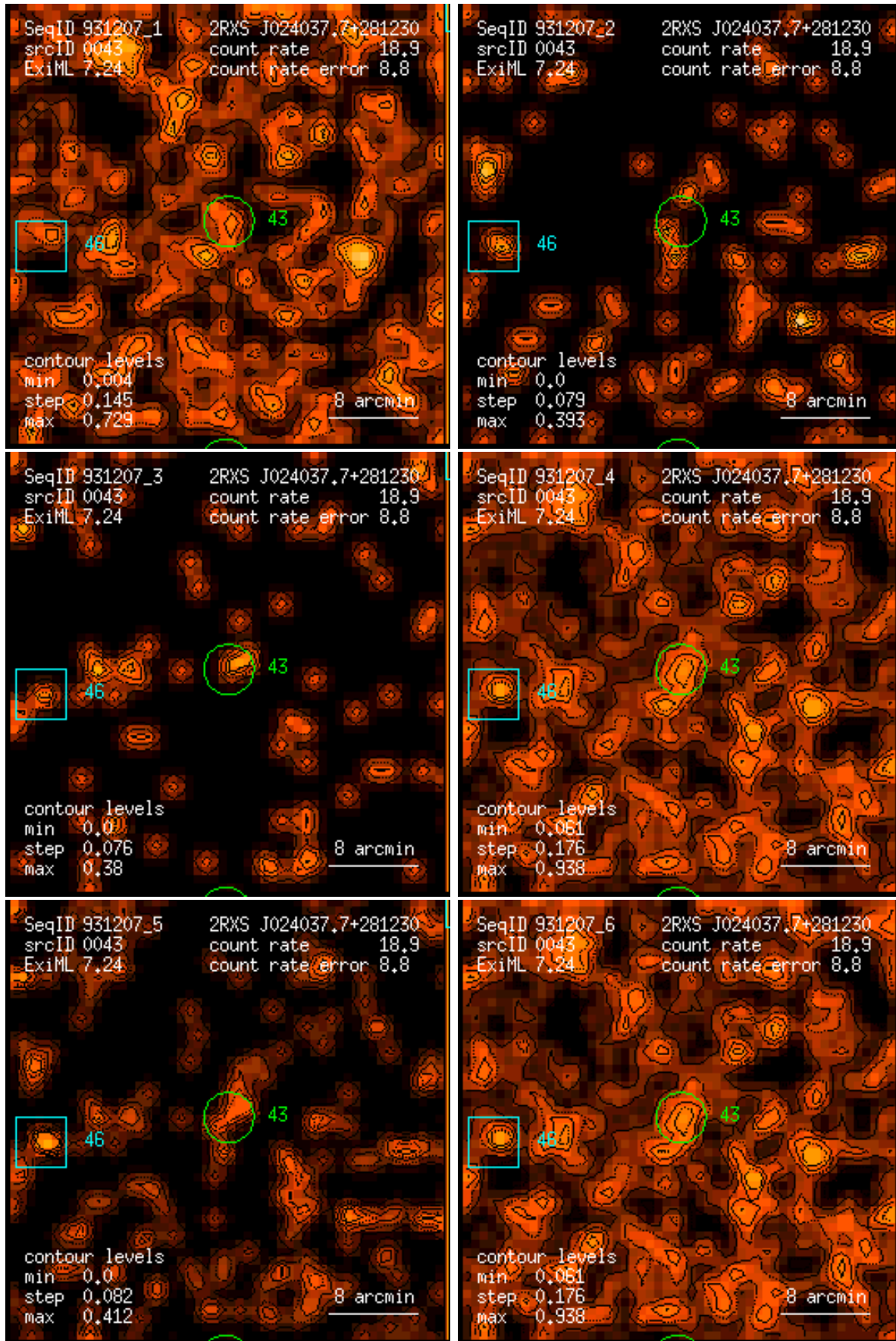
Figure 43: RASS 931207: detection 0043: band rate images, Gaussian filter: (1) PSPC channels 11 – 41, (2) 52 – 90, (3) 91 – 201, (4) 11 – 235, (5) 52 – 201, (6) 11 – 201. Broad band rates in counts/ks. Band rate contour levels in counts/ks/arcmin 2 .
