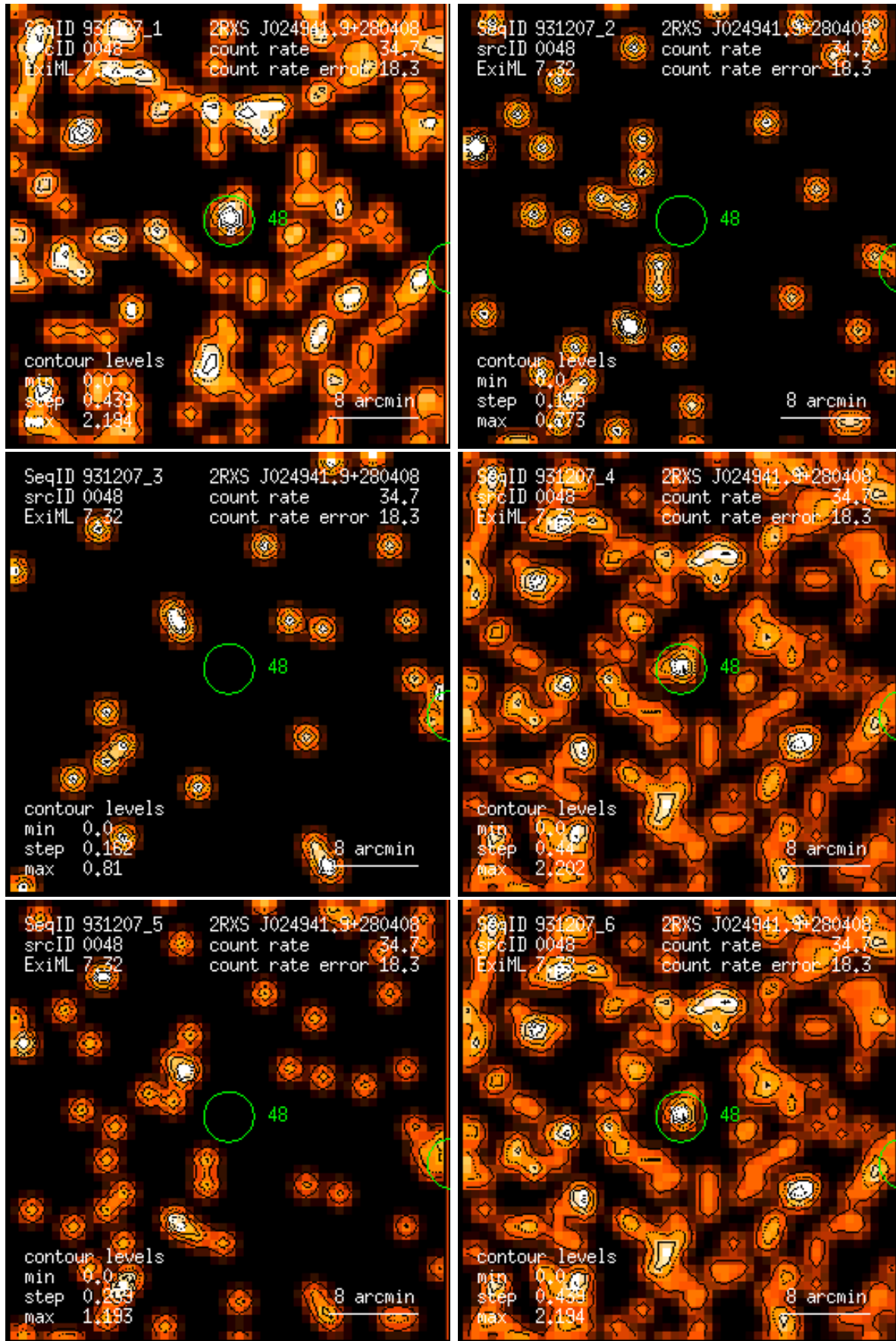
Figure 48: RASS 931207: detection 0048: band rate images, Gaussian filter: (1) PSPC channels 11 – 41, (2) 52 – 90, (3) 91 – 201, (4) 11 – 235, (5) 52 – 201, (6) 11 – 201. Broad band rates in counts/ks. Band rate contour levels in counts/ks/arcmin 2 .
