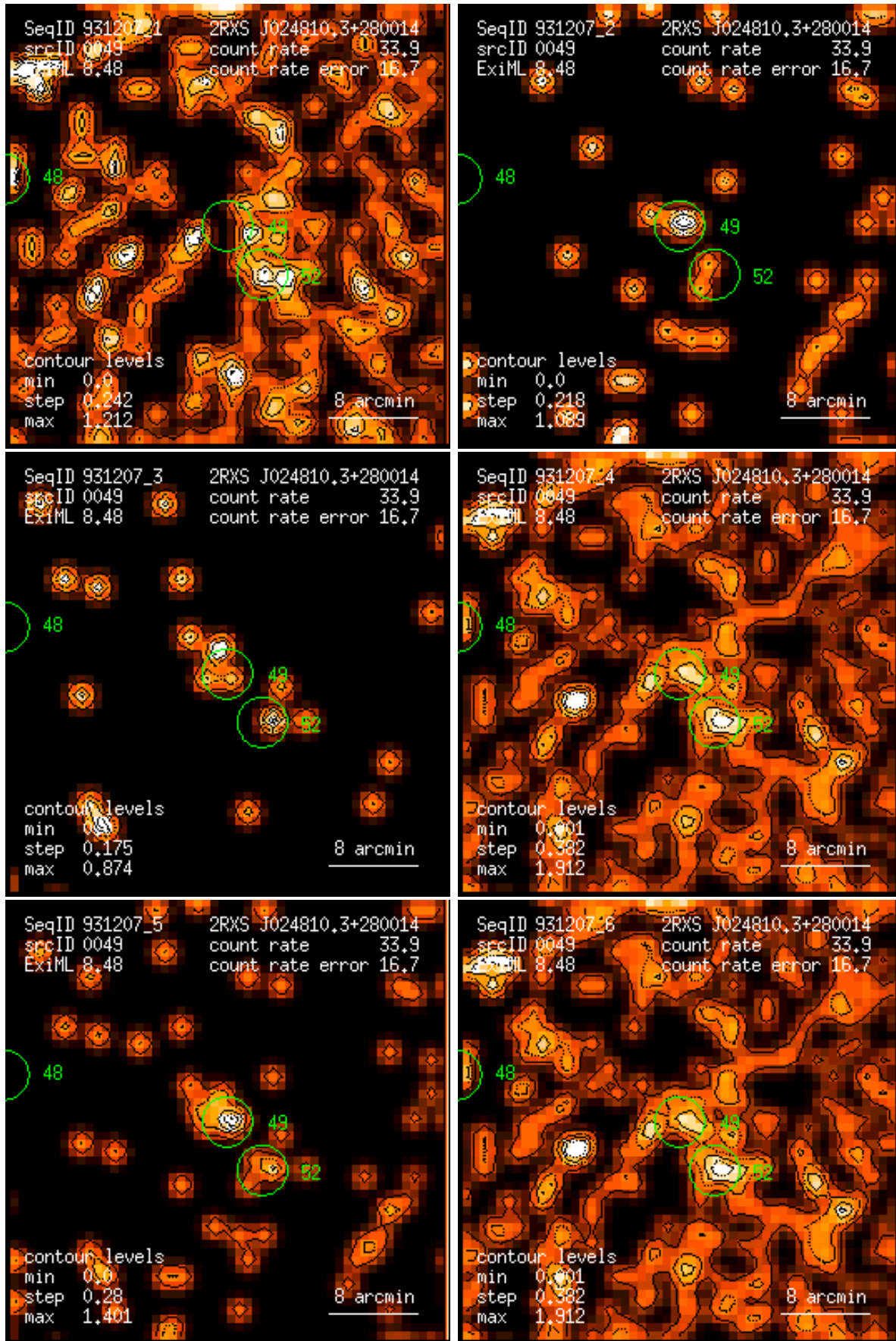
Figure 49: RASS 931207: detection 0049: band rate images, Gaussian filter: (1) PSPC channels 11 – 41, (2) 52 – 90, (3) 91 – 201, (4) 11 – 235, (5) 52 – 201, (6) 11 – 201. Broad band rates in counts/ks. Band rate contour levels in counts/ks/arcmin 2 .
