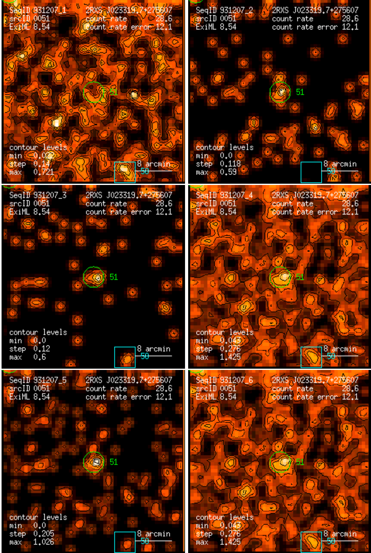
Figure 51: RASS 931207: detection 0051: band rate images, Gaussian filter: (1) PSPC channels 11 – 41, (2) 52 – 90, (3) 91 – 201, (4) 11 – 235, (5) 52 – 201, (6) 11 – 201. Broad band rates in counts/ks. Band rate contour levels in counts/ks/arcmin 2 .
