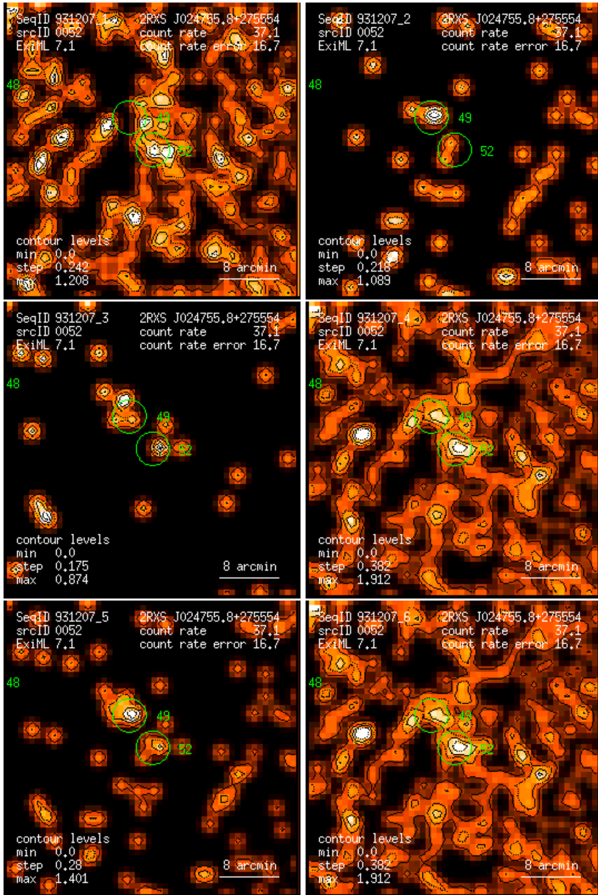
Figure 52: RASS 931207: detection 0052: band rate images, Gaussian filter: (1) PSPC channels 11 – 41, (2) 52 – 90, (3) 91 – 201, (4) 11 – 235, (5) 52 – 201, (6) 11 – 201. Broad band rates in counts/ks. Band rate contour levels in counts/ks/arcmin 2 .
