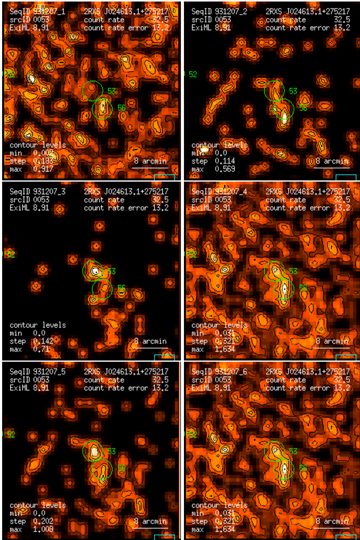
Figure 53: RASS 931207: detection 0053: band rate images, Gaussian filter: (1) PSPC channels 11 – 41, (2) 52 – 90, (3) 91 – 201, (4) 11 – 235, (5) 52 – 201, (6) 11 – 201. Broad band rates in counts/ks. Band rate contour levels in counts/ks/arcmin 2 .
