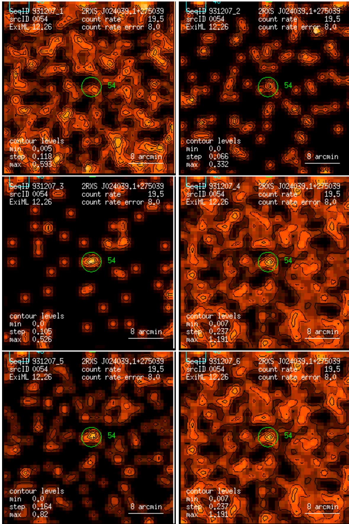
Figure 54: RASS 931207: detection 0054: band rate images, Gaussian filter: (1) PSPC channels 11 – 41, (2) 52 – 90, (3) 91 – 201, (4) 11 – 235, (5) 52 – 201, (6) 11 – 201. Broad band rates in counts/ks. Band rate contour levels in counts/ks/arcmin 2 .
