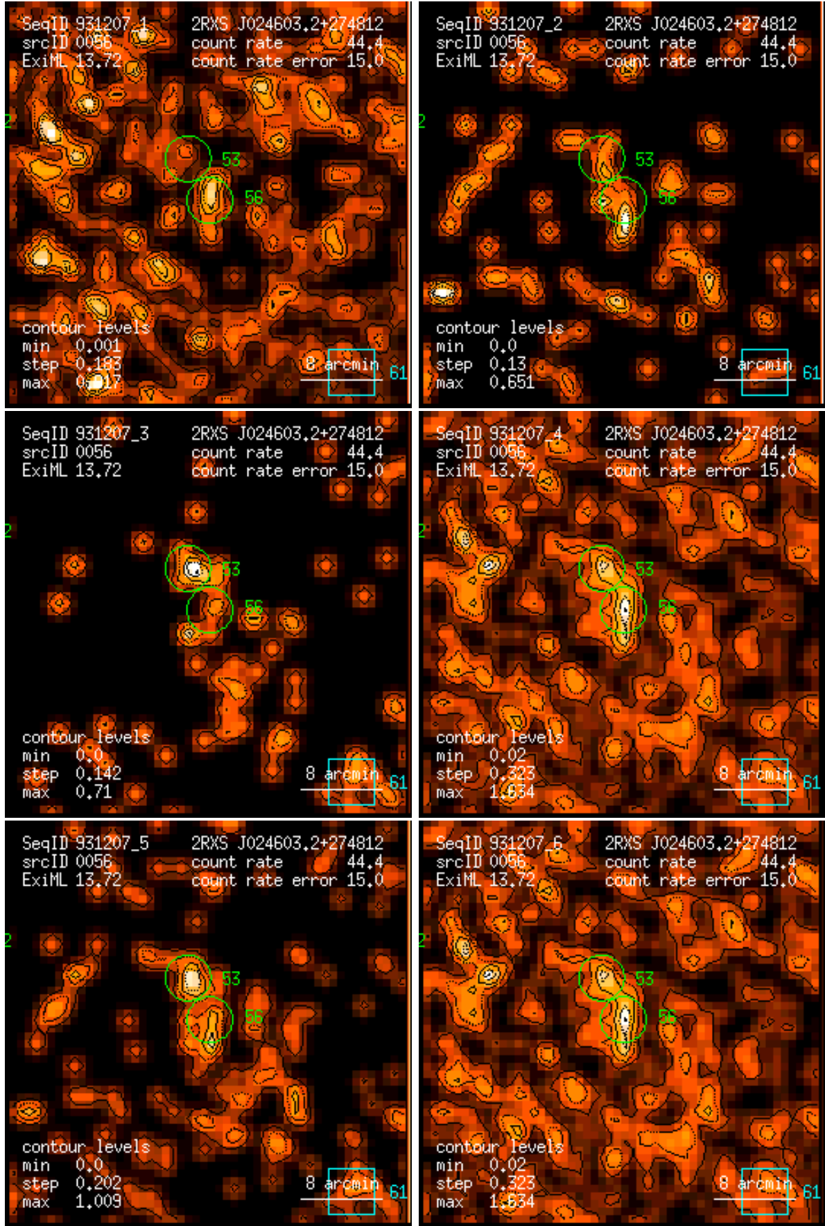
Figure 56: RASS 931207: detection 0056: band rate images, Gaussian filter: (1) PSPC channels 11 – 41, (2) 52 – 90, (3) 91 – 201, (4) 11 – 235, (5) 52 – 201, (6) 11 – 201. Broad band rates in counts/ks. Band rate contour levels in counts/ks/arcmin 2 .
