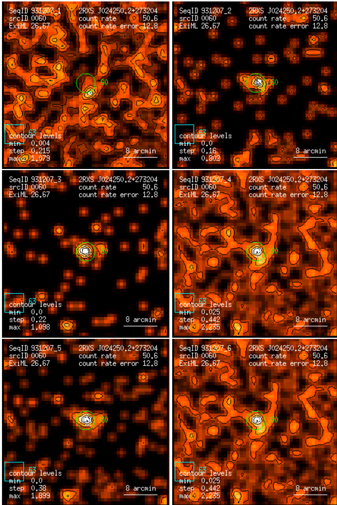
Figure 60: RASS 931207: detection 0060: band rate images, Gaussian filter: (1) PSPC channels 11 – 41, (2) 52 – 90, (3) 91 – 201, (4) 11 – 235, (5) 52 – 201, (6) 11 – 201. Broad band rates in counts/ks. Band rate contour levels in counts/ks/arcmin 2 .
