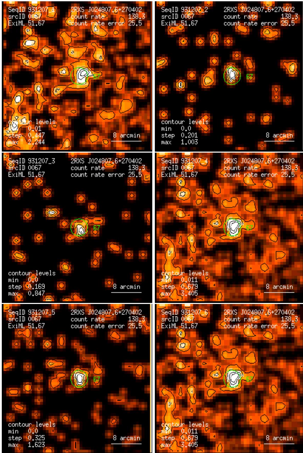
Figure 67: RASS 931207: detection 0067: band rate images, Gaussian filter: (1) PSPC channels 11 – 41, (2) 52 – 90, (3) 91 – 201, (4) 11 – 235, (5) 52 – 201, (6) 11 – 201. Broad band rates in counts/ks. Band rate contour levels in counts/ks/arcmin 2 .
