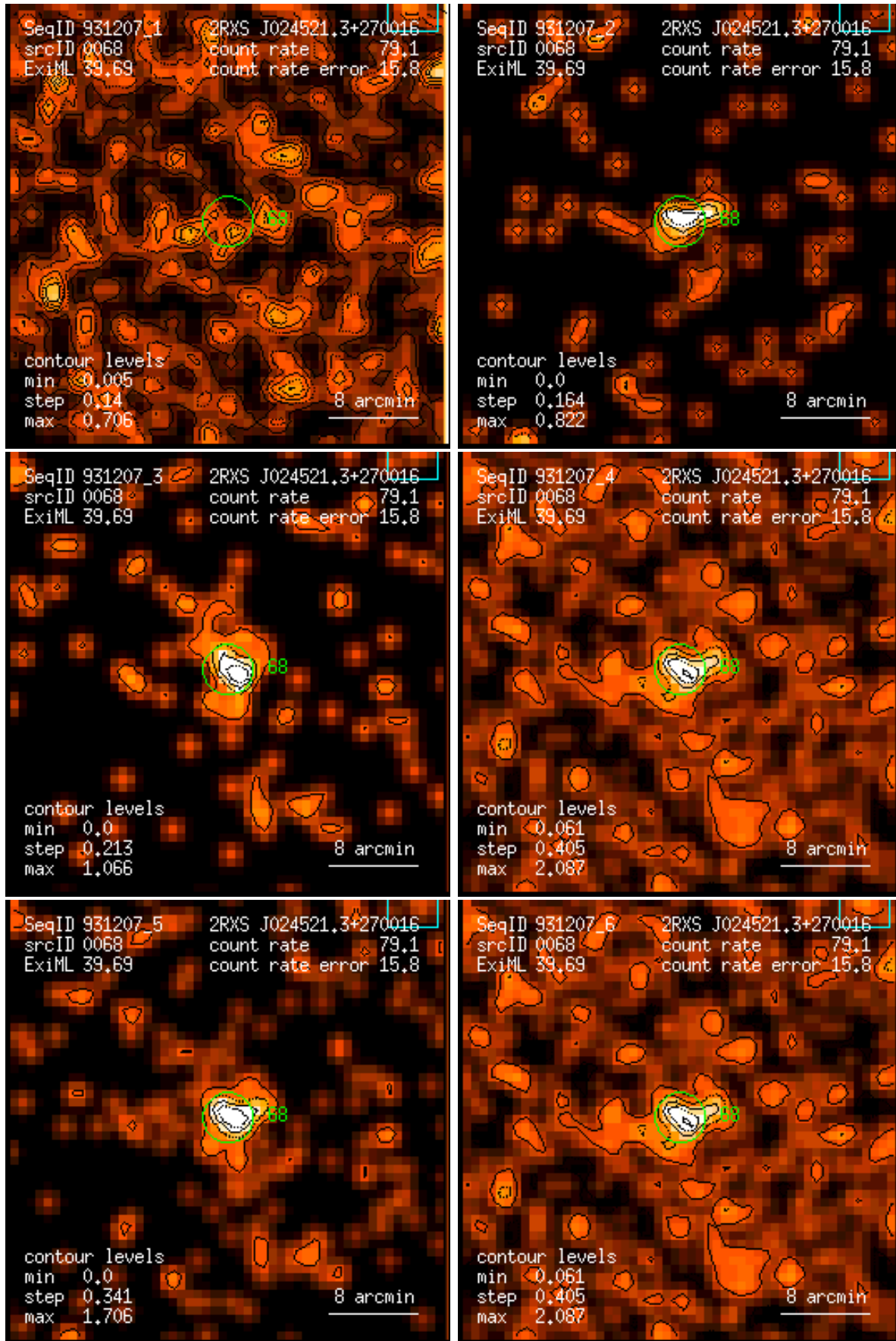
Figure 68: RASS 931207: detection 0068: band rate images, Gaussian filter: (1) PSPC channels 11 – 41, (2) 52 – 90, (3) 91 – 201, (4) 11 – 235, (5) 52 – 201, (6) 11 – 201. Broad band rates in counts/ks. Band rate contour levels in counts/ks/arcmin 2 .
