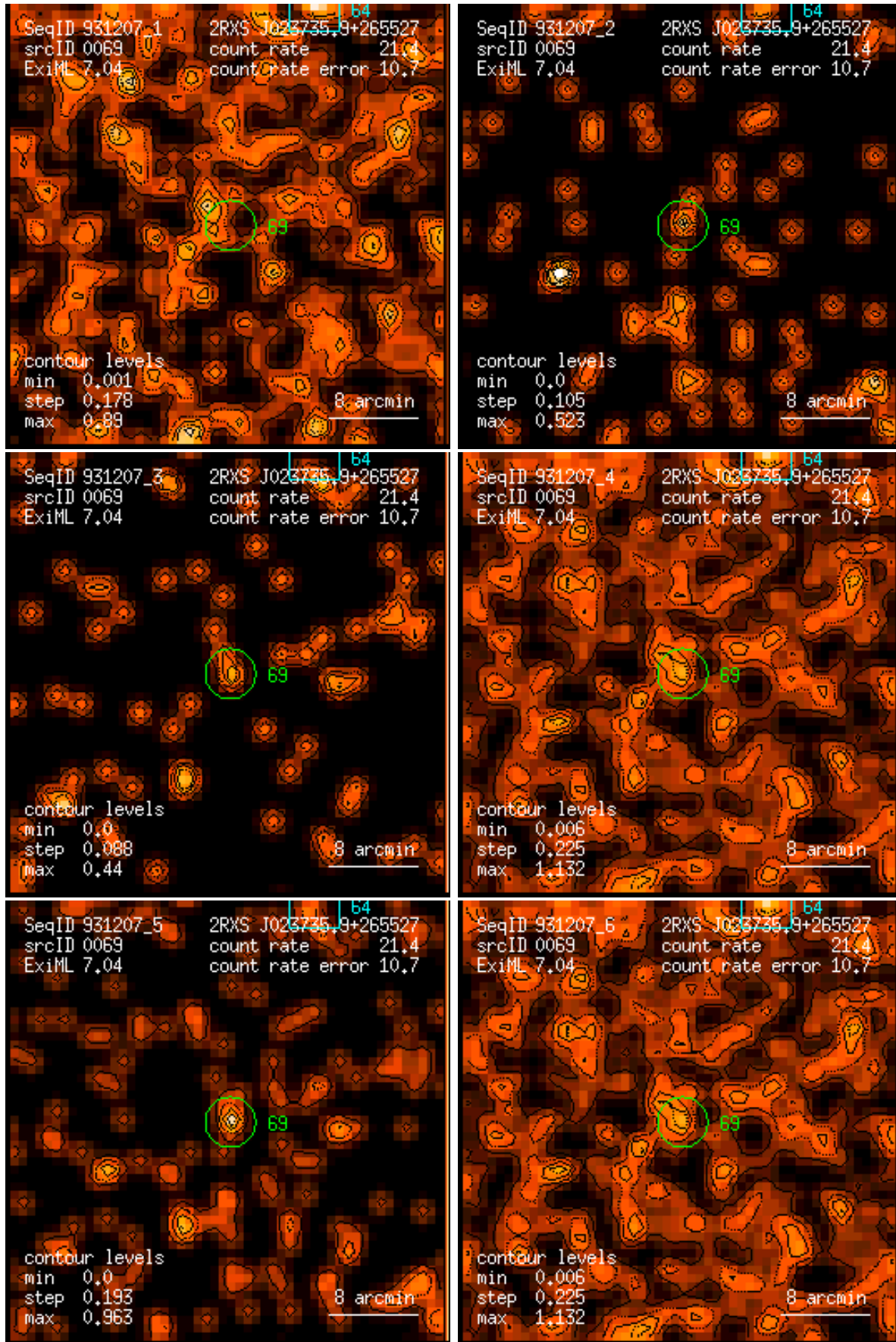
Figure 69: RASS 931207: detection 0069: band rate images, Gaussian filter: (1) PSPC channels 11 – 41, (2) 52 – 90, (3) 91 – 201, (4) 11 – 235, (5) 52 – 201, (6) 11 – 201. Broad band rates in counts/ks. Band rate contour levels in counts/ks/arcmin 2 .
