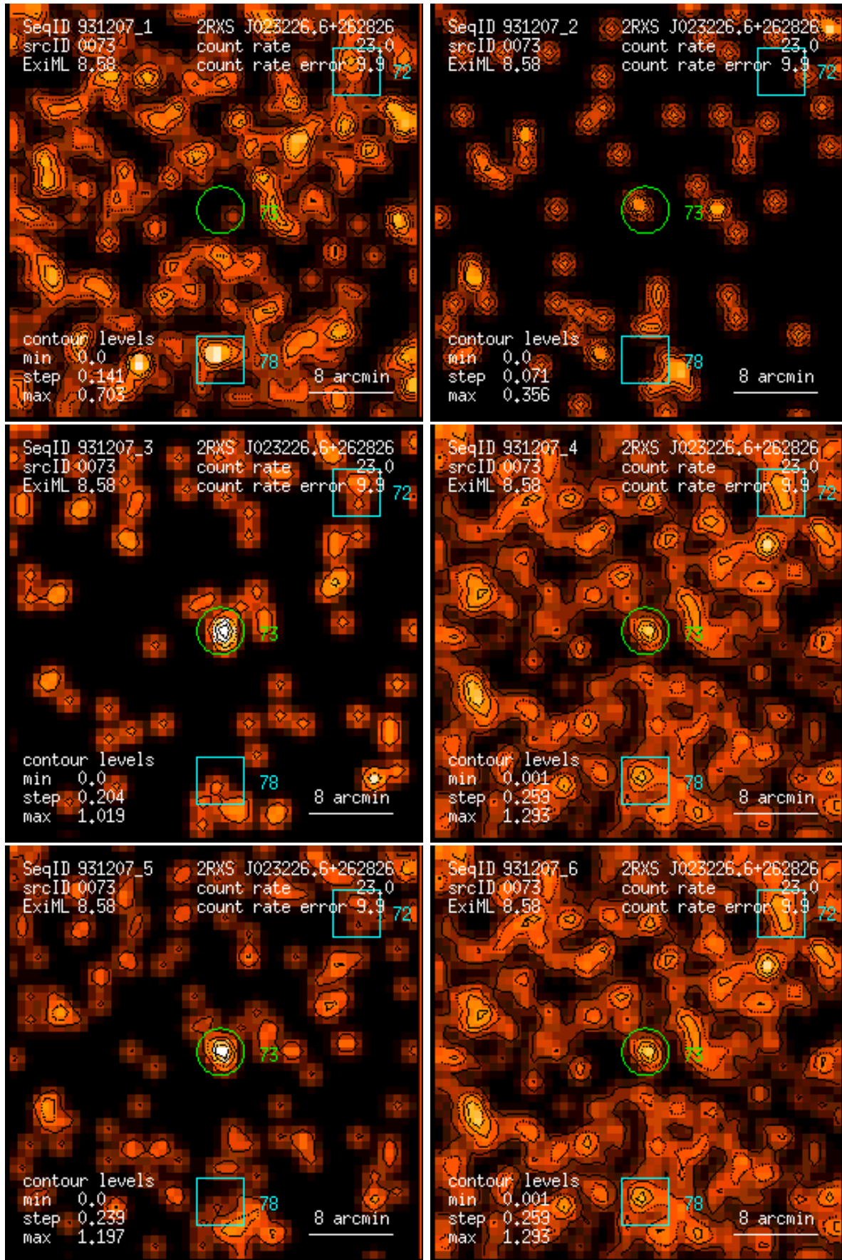
Figure 73: RASS 931207: detection 0073: band rate images, Gaussian filter: (1) PSPC channels 11 – 41, (2) 52 – 90, (3) 91 – 201, (4) 11 – 235, (5) 52 – 201, (6) 11 – 201. Broad band rates in counts/ks. Band rate contour levels in counts/ks/arcmin 2 .
