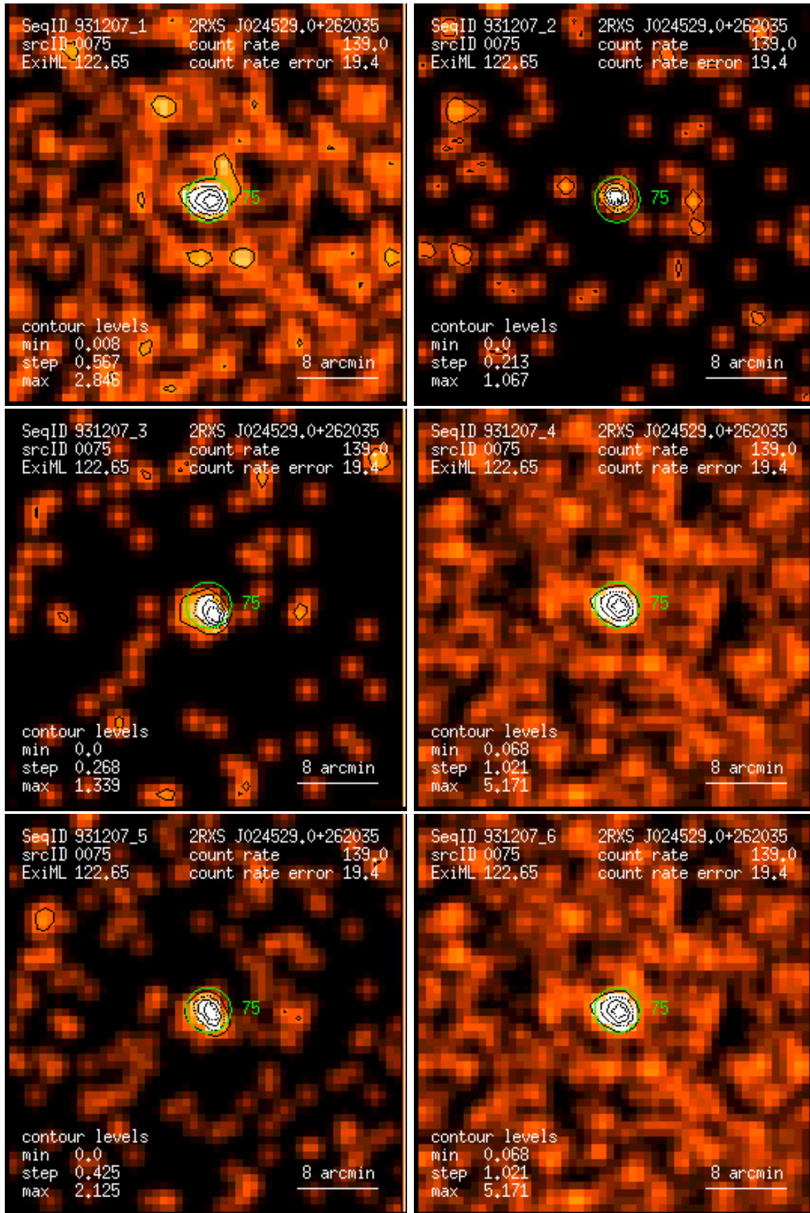
Figure 75: RASS 931207: detection 0075: band rate images, Gaussian filter: (1) PSPC channels 11 – 41, (2) 52 – 90, (3) 91 – 201, (4) 11 – 235, (5) 52 – 201, (6) 11 – 201. Broad band rates in counts/ks. Band rate contour levels in counts/ks/arcmin 2 .
