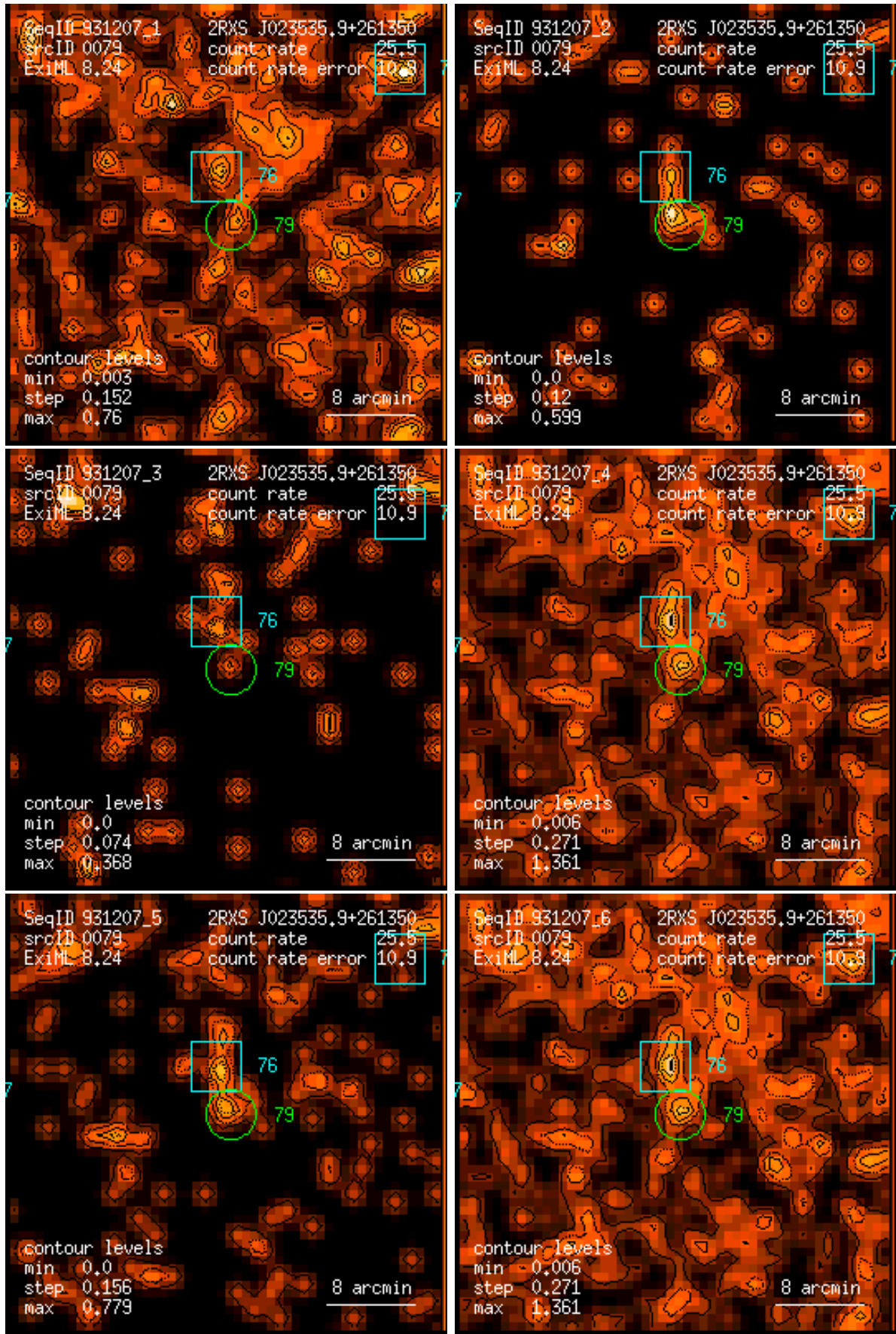
Figure 79: RASS 931207: detection 0079: band rate images, Gaussian filter: (1) PSPC channels 11 – 41, (2) 52 – 90, (3) 91 – 201, (4) 11 – 235, (5) 52 – 201, (6) 11 – 201. Broad band rates in counts/ks. Band rate contour levels in counts/ks/arcmin 2 .
