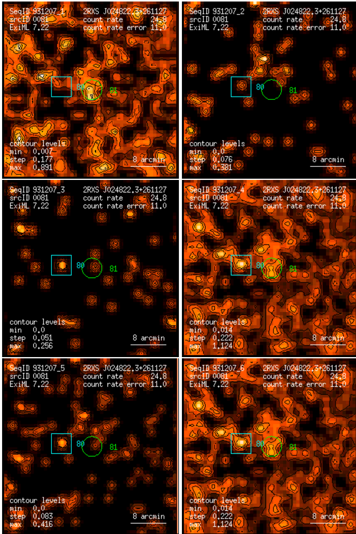
Figure 81: RASS 931207: detection 0081: band rate images, Gaussian filter: (1) PSPC channels 11 – 41, (2) 52 – 90, (3) 91 – 201, (4) 11 – 235, (5) 52 – 201, (6) 11 – 201. Broad band rates in counts/ks. Band rate contour levels in counts/ks/arcmin 2 .
