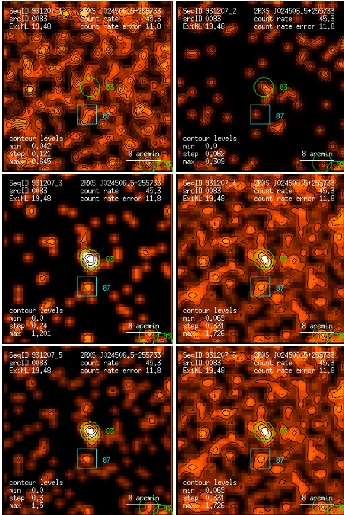
Figure 83: RASS 931207: detection 0083: band rate images, Gaussian filter: (1) PSPC channels 11 – 41, (2) 52 – 90, (3) 91 – 201, (4) 11 – 235, (5) 52 – 201, (6) 11 – 201. Broad band rates in counts/ks. Band rate contour levels in counts/ks/arcmin 2 .
