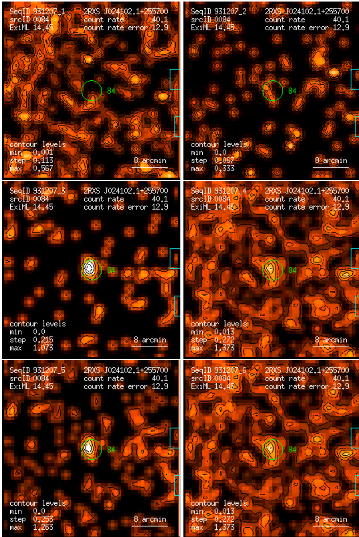
Figure 84: RASS 931207: detection 0084: band rate images, Gaussian filter: (1) PSPC channels 11 – 41, (2) 52 – 90, (3) 91 – 201, (4) 11 – 235, (5) 52 – 201, (6) 11 – 201. Broad band rates in counts/ks. Band rate contour levels in counts/ks/arcmin 2 .
