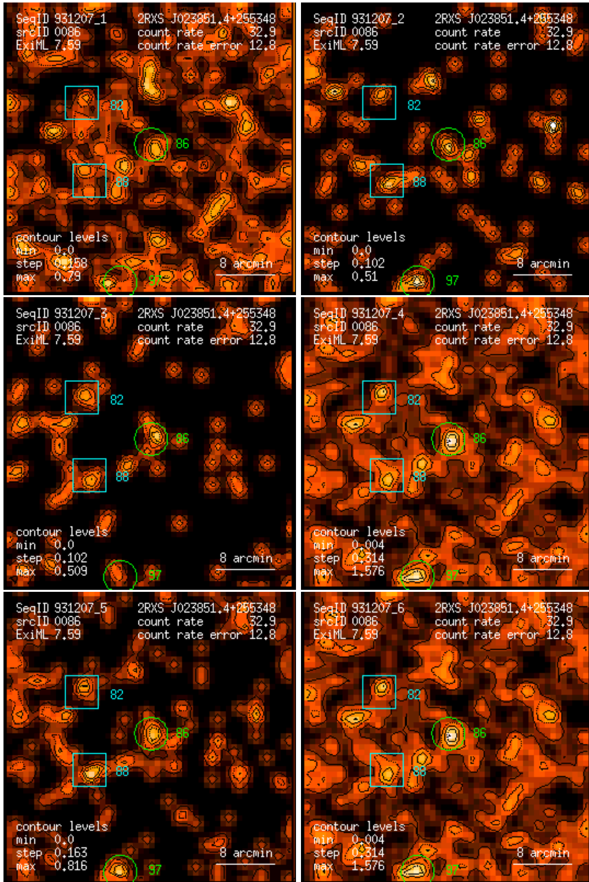
Figure 86: RASS 931207: detection 0086: band rate images, Gaussian filter: (1) PSPC channels 11 – 41, (2) 52 – 90, (3) 91 – 201, (4) 11 – 235, (5) 52 – 201, (6) 11 – 201. Broad band rates in counts/ks. Band rate contour levels in counts/ks/arcmin 2 .
