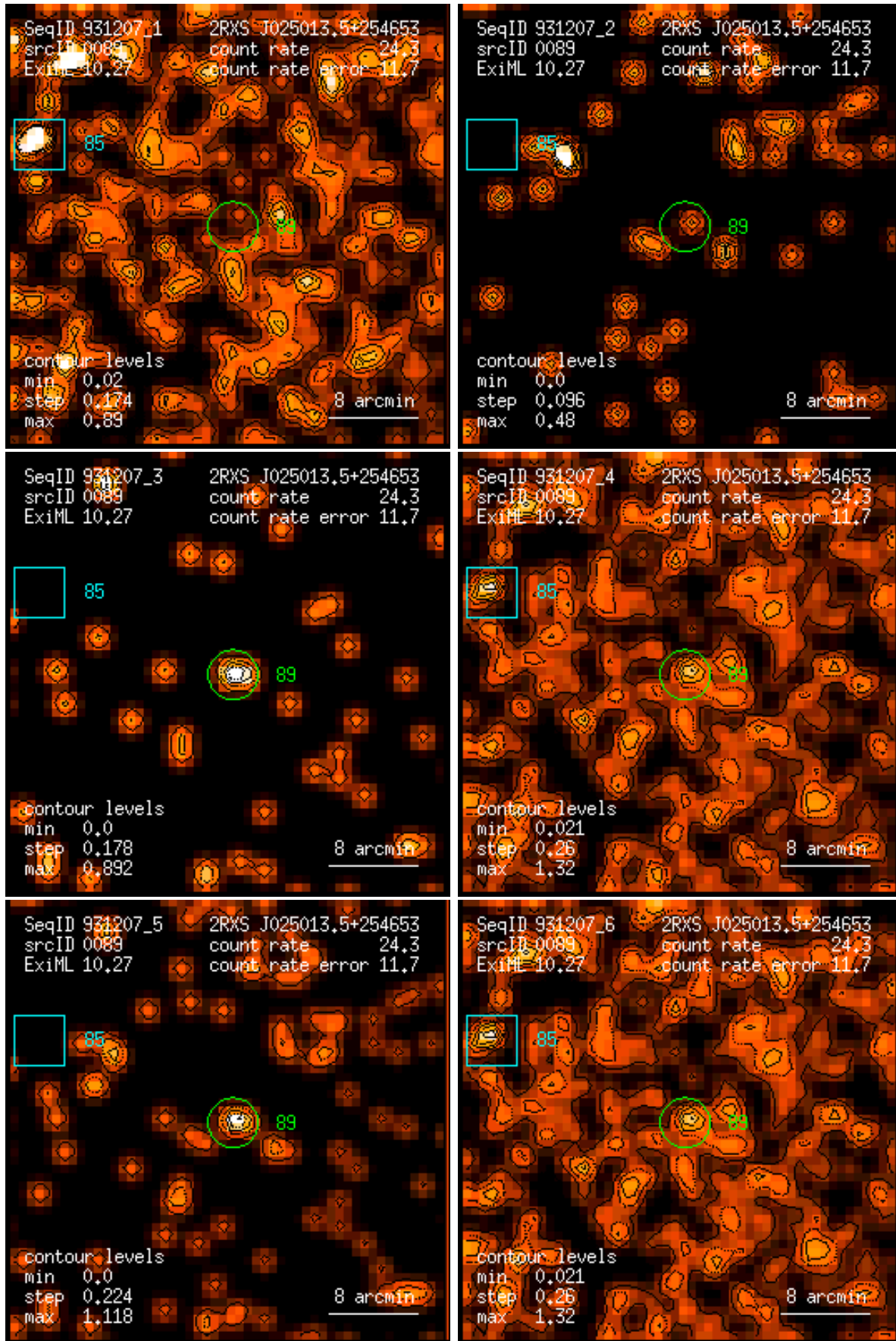
Figure 89: RASS 931207: detection 0089: band rate images, Gaussian filter: (1) PSPC channels 11 – 41, (2) 52 – 90, (3) 91 – 201, (4) 11 – 235, (5) 52 – 201, (6) 11 – 201. Broad band rates in counts/ks. Band rate contour levels in counts/ks/arcmin 2 .
