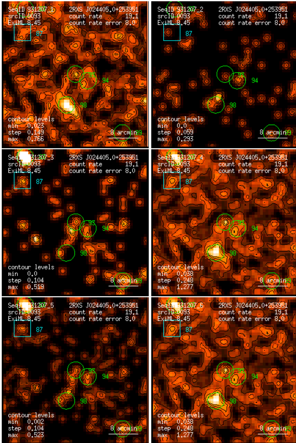
Figure 93: RASS 931207: detection 0093: band rate images, Gaussian filter: (1) PSPC channels 11 – 41, (2) 52 – 90, (3) 91 – 201, (4) 11 – 235, (5) 52 – 201, (6) 11 – 201. Broad band rates in counts/ks. Band rate contour levels in counts/ks/arcmin 2 .
