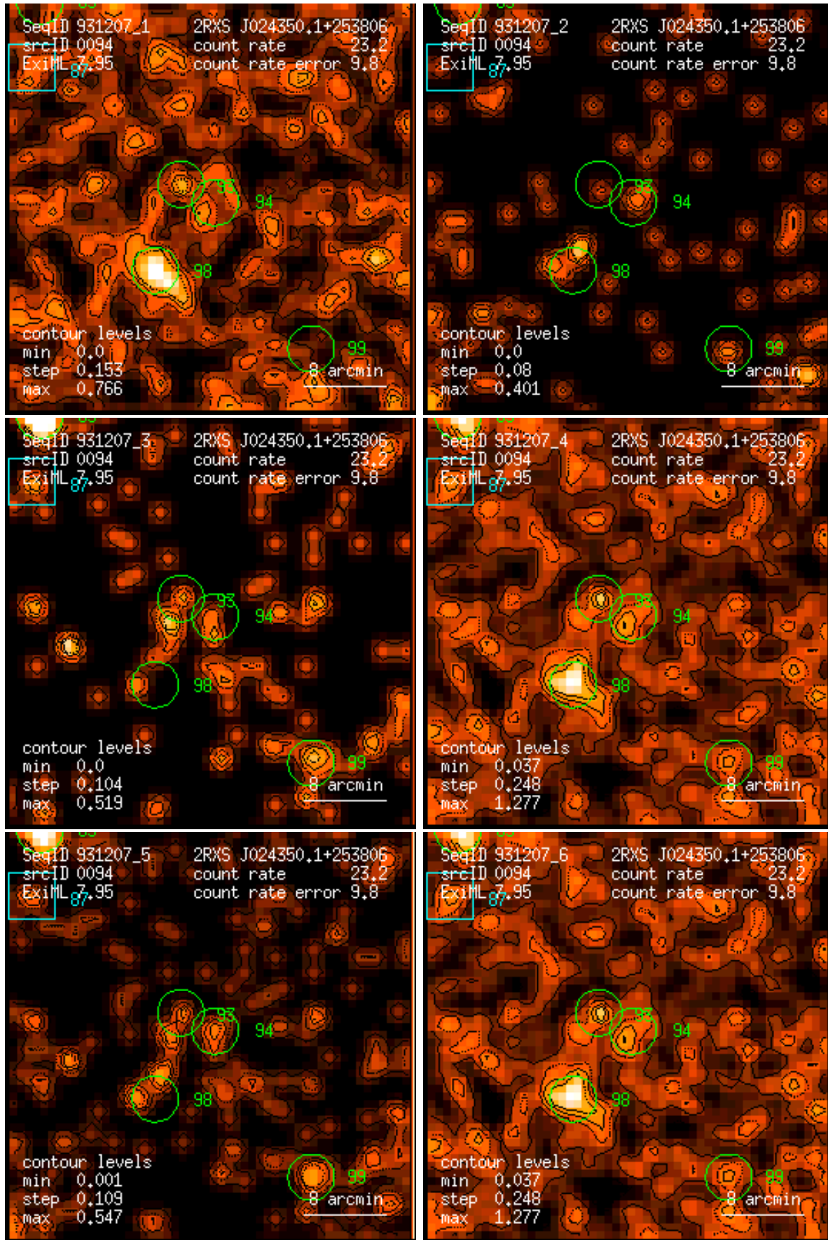
Figure 94: RASS 931207: detection 0094: band rate images, Gaussian filter: (1) PSPC channels 11 – 41, (2) 52 – 90, (3) 91 – 201, (4) 11 – 235, (5) 52 – 201, (6) 11 – 201. Broad band rates in counts/ks. Band rate contour levels in counts/ks/arcmin 2 .
