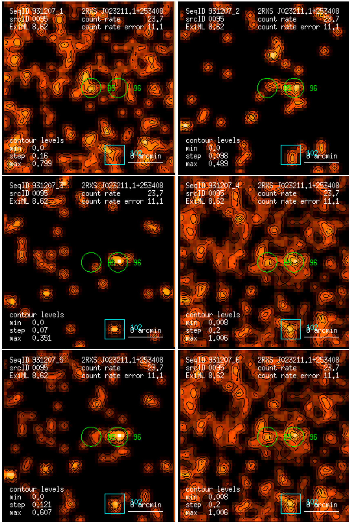
Figure 95: RASS 931207: detection 0095: band rate images, Gaussian filter: (1) PSPC channels 11 – 41, (2) 52 – 90, (3) 91 – 201, (4) 11 – 235, (5) 52 – 201, (6) 11 – 201. Broad band rates in counts/ks. Band rate contour levels in counts/ks/arcmin 2 .
