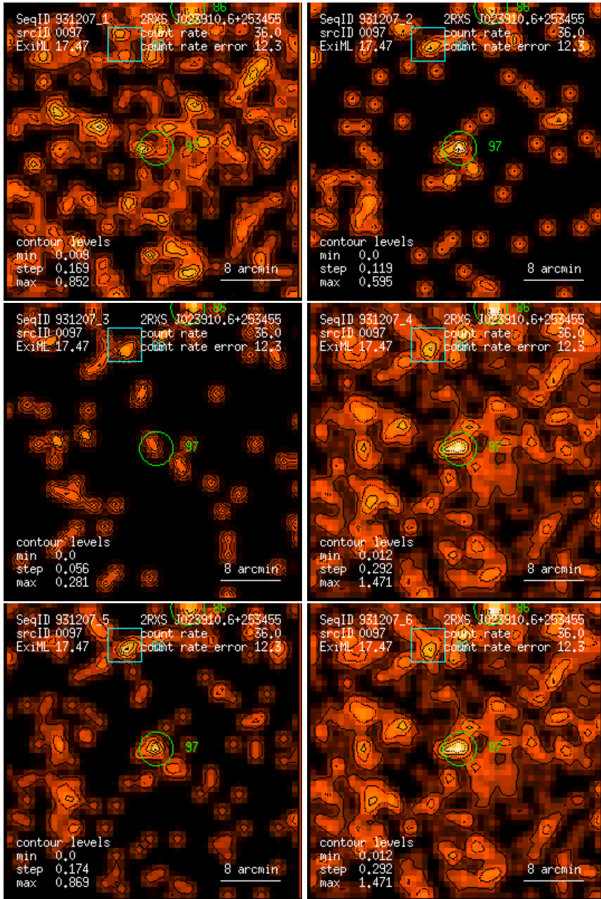
Figure 97: RASS 931207: detection 0097: band rate images, Gaussian filter: (1) PSPC channels 11 – 41, (2) 52 – 90, (3) 91 – 201, (4) 11 – 235, (5) 52 – 201, (6) 11 – 201. Broad band rates in counts/ks. Band rate contour levels in counts/ks/arcmin 2 .
