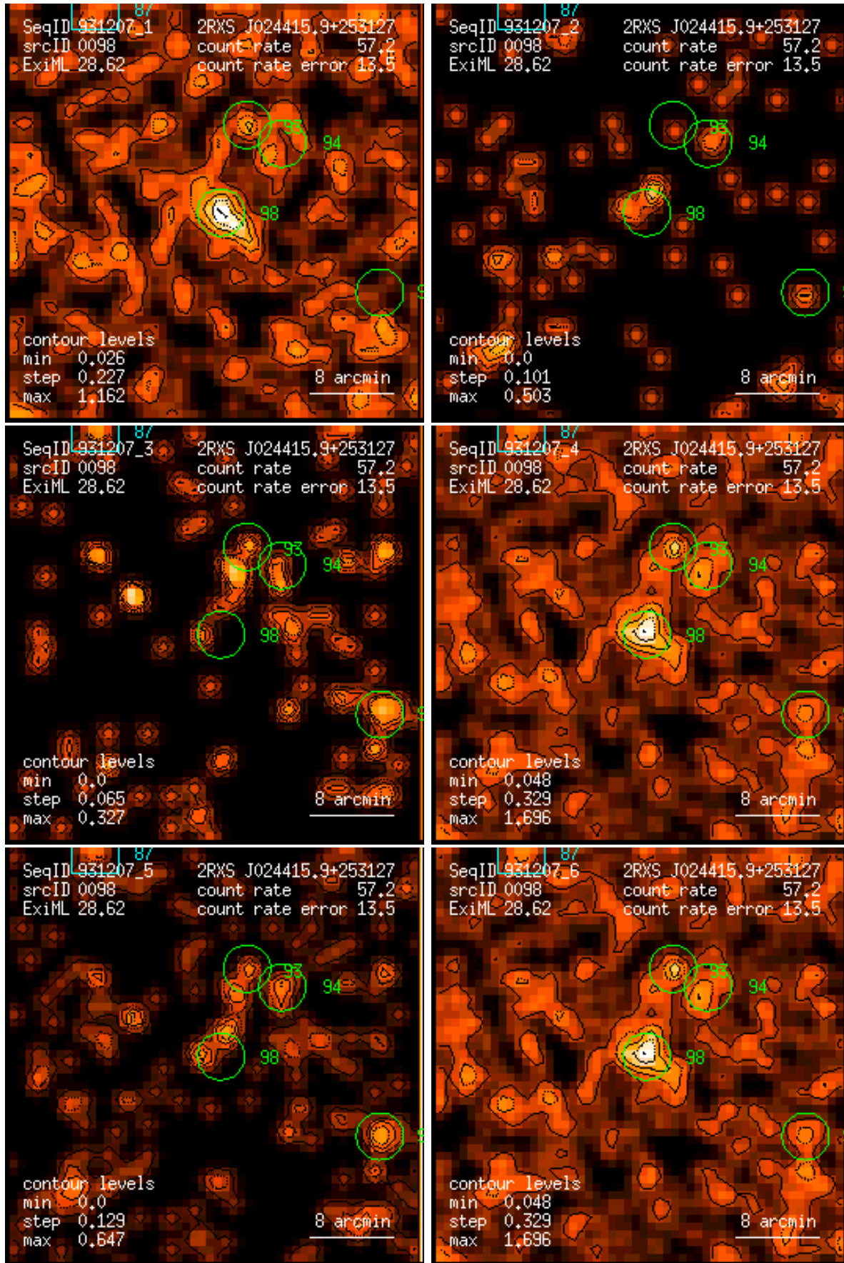
Figure 98: RASS 931207: detection 0098: band rate images, Gaussian filter: (1) PSPC channels 11 – 41, (2) 52 – 90, (3) 91 – 201, (4) 11 – 235, (5) 52 – 201, (6) 11 – 201. Broad band rates in counts/ks. Band rate contour levels in counts/ks/arcmin 2 .
