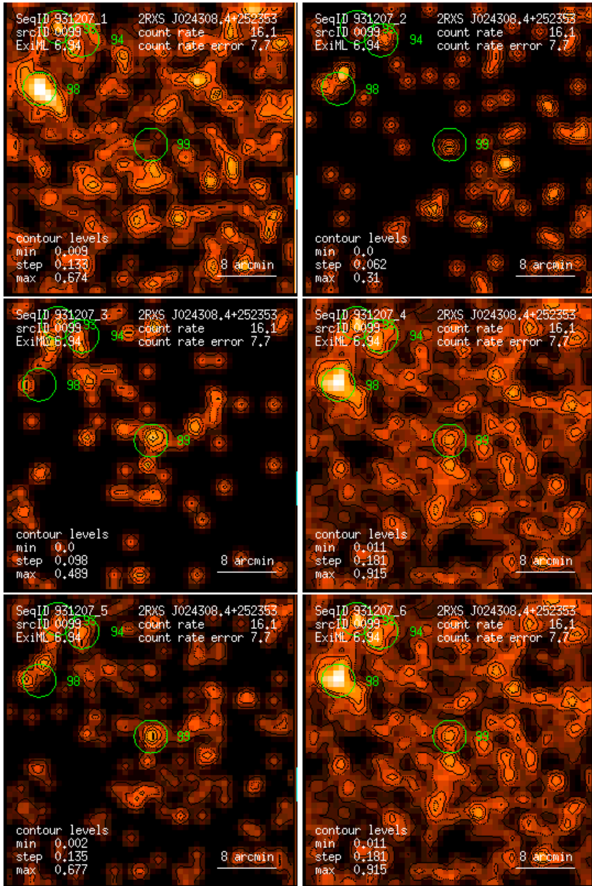
Figure 99: RASS 931207: detection 0099: band rate images, Gaussian filter: (1) PSPC channels 11 – 41, (2) 52 – 90, (3) 91 – 201, (4) 11 – 235, (5) 52 – 201, (6) 11 – 201. Broad band rates in counts/ks. Band rate contour levels in counts/ks/arcmin 2 .
