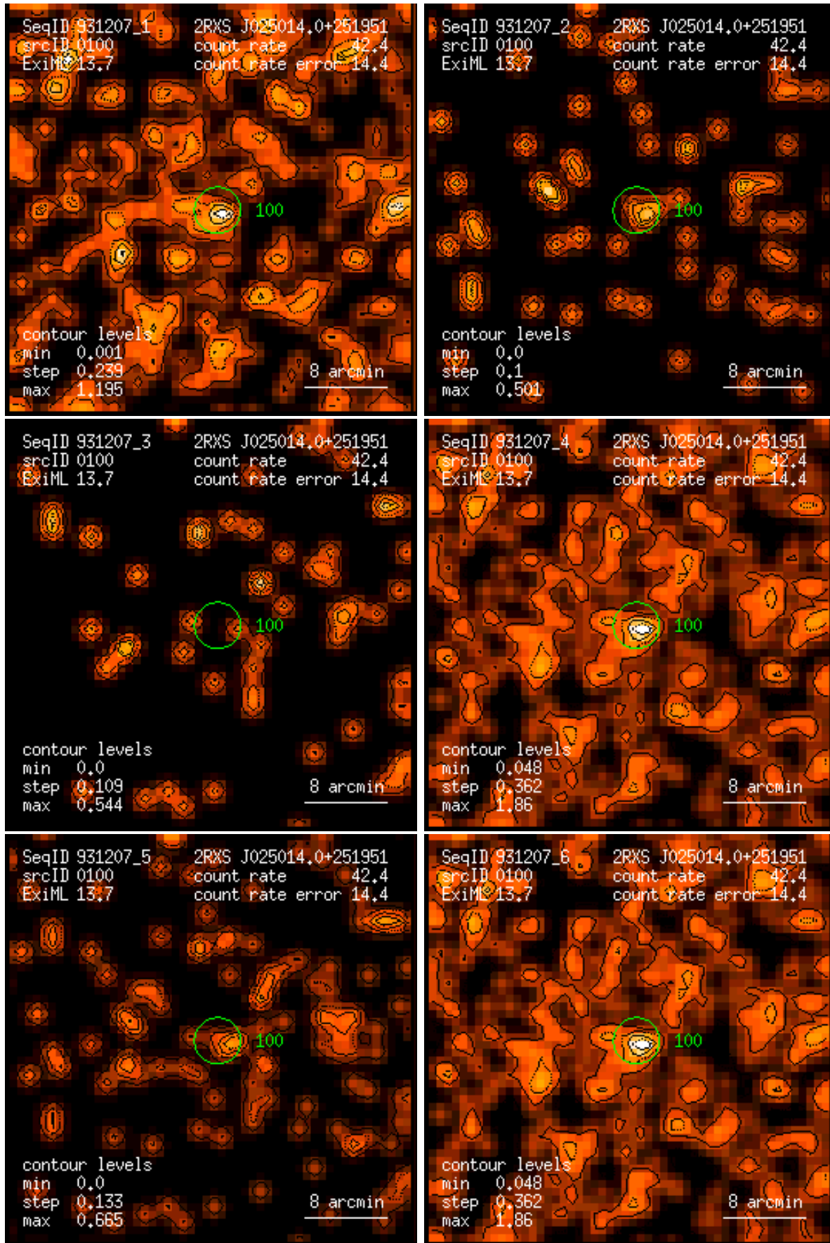
Figure 100: RASS 931207: detection 0100: band rate images, Gaussian filter: (1) PSPC channels 11 – 41, (2) 52 – 90, (3) 91 – 201, (4) 11 – 235, (5) 52 – 201, (6) 11 – 201. Broad band rates in counts/ks. Band rate contour levels in counts/ks/arcmin 2 .
