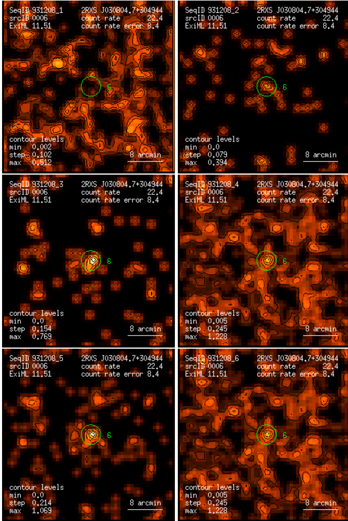
Figure 6: RASS 931208: detection 0006: band rate images, Gaussian filter: (1) PSPC channels 11 – 41, (2) 52 – 90, (3) 91 – 201, (4) 11 – 235, (5) 52 – 201, (6) 11 – 201. Broad band rates in counts/ks. Band rate contour levels in counts/ks/arcmin 2 .
