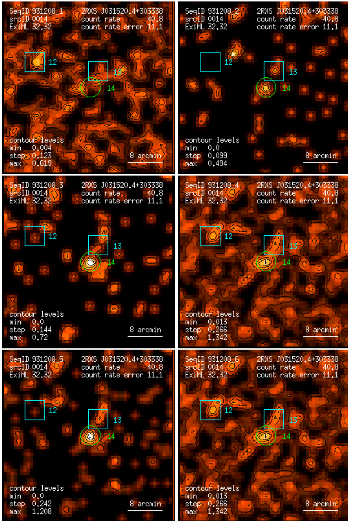
Figure 14: RASS 931208: detection 0014: band rate images, Gaussian filter: (1) PSPC channels 11 – 41, (2) 52 – 90, (3) 91 – 201, (4) 11 – 235, (5) 52 – 201, (6) 11 – 201. Broad band rates in counts/ks. Band rate contour levels in counts/ks/arcmin 2 .
