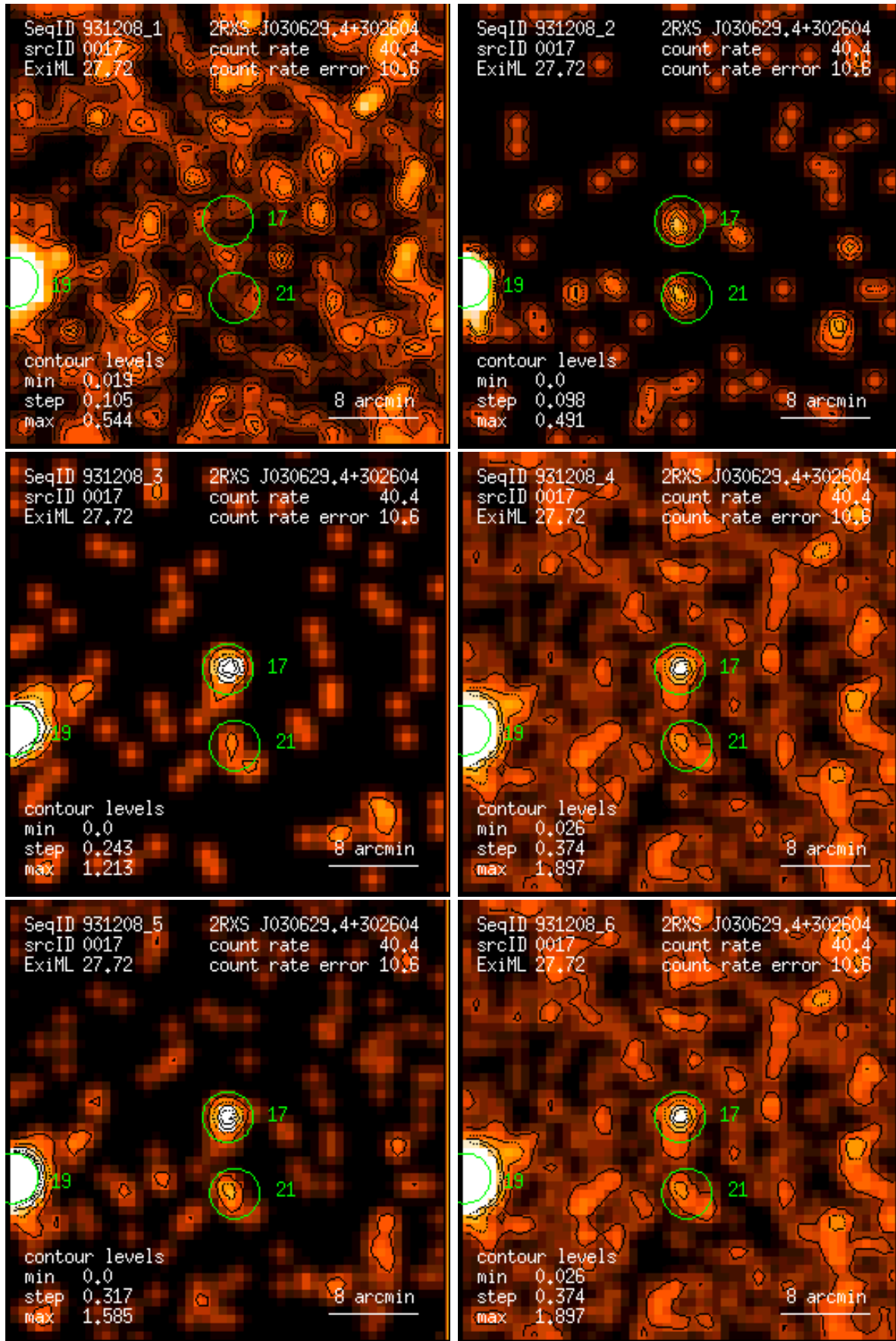
Figure 17: RASS 931208: detection 0017: band rate images, Gaussian filter: (1) PSPC channels 11 – 41, (2) 52 – 90, (3) 91 – 201, (4) 11 – 235, (5) 52 – 201, (6) 11 – 201. Broad band rates in counts/ks. Band rate contour levels in counts/ks/arcmin 2 .
