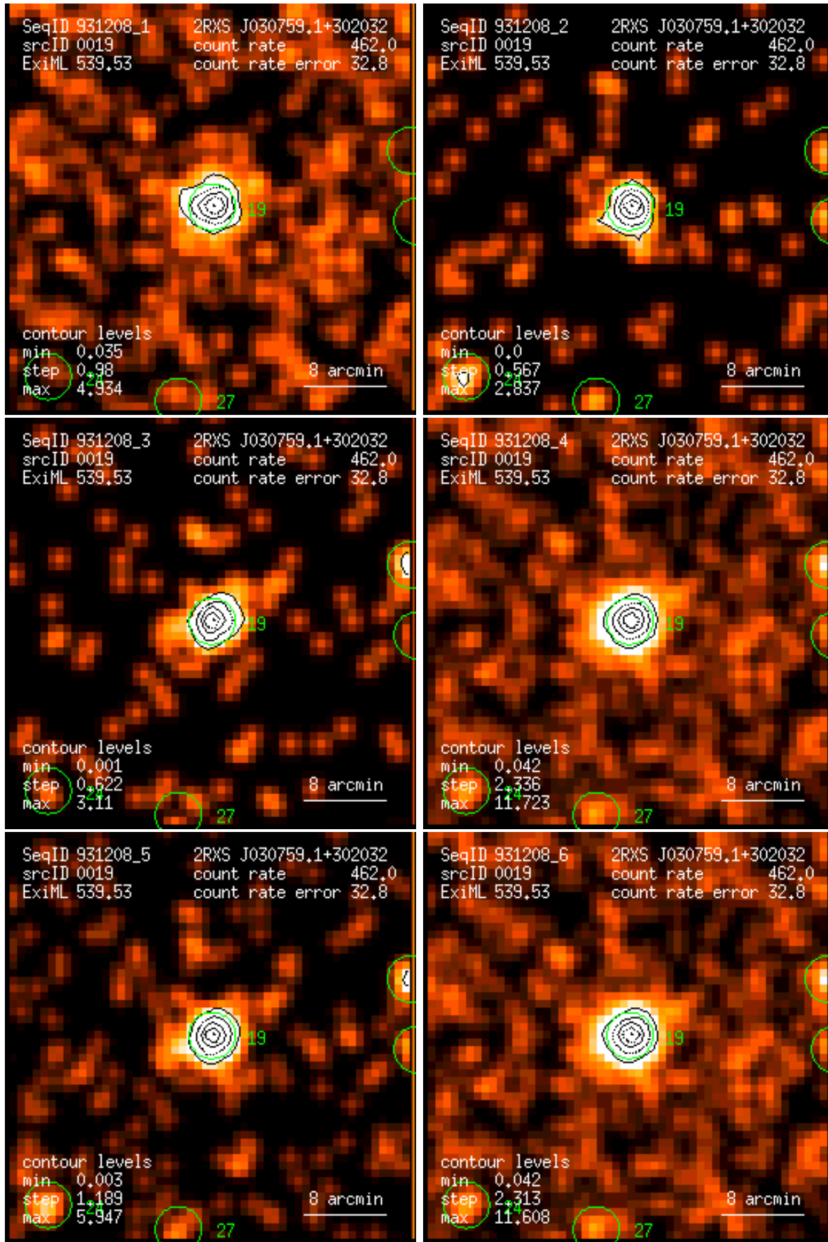
Figure 19: RASS 931208: detection 0019: band rate images, Gaussian filter: (1) PSPC channels 11 – 41, (2) 52 – 90, (3) 91 – 201, (4) 11 – 235, (5) 52 – 201, (6) 11 – 201. Broad band rates in counts/ks. Band rate contour levels in counts/ks/arcmin 2 .
