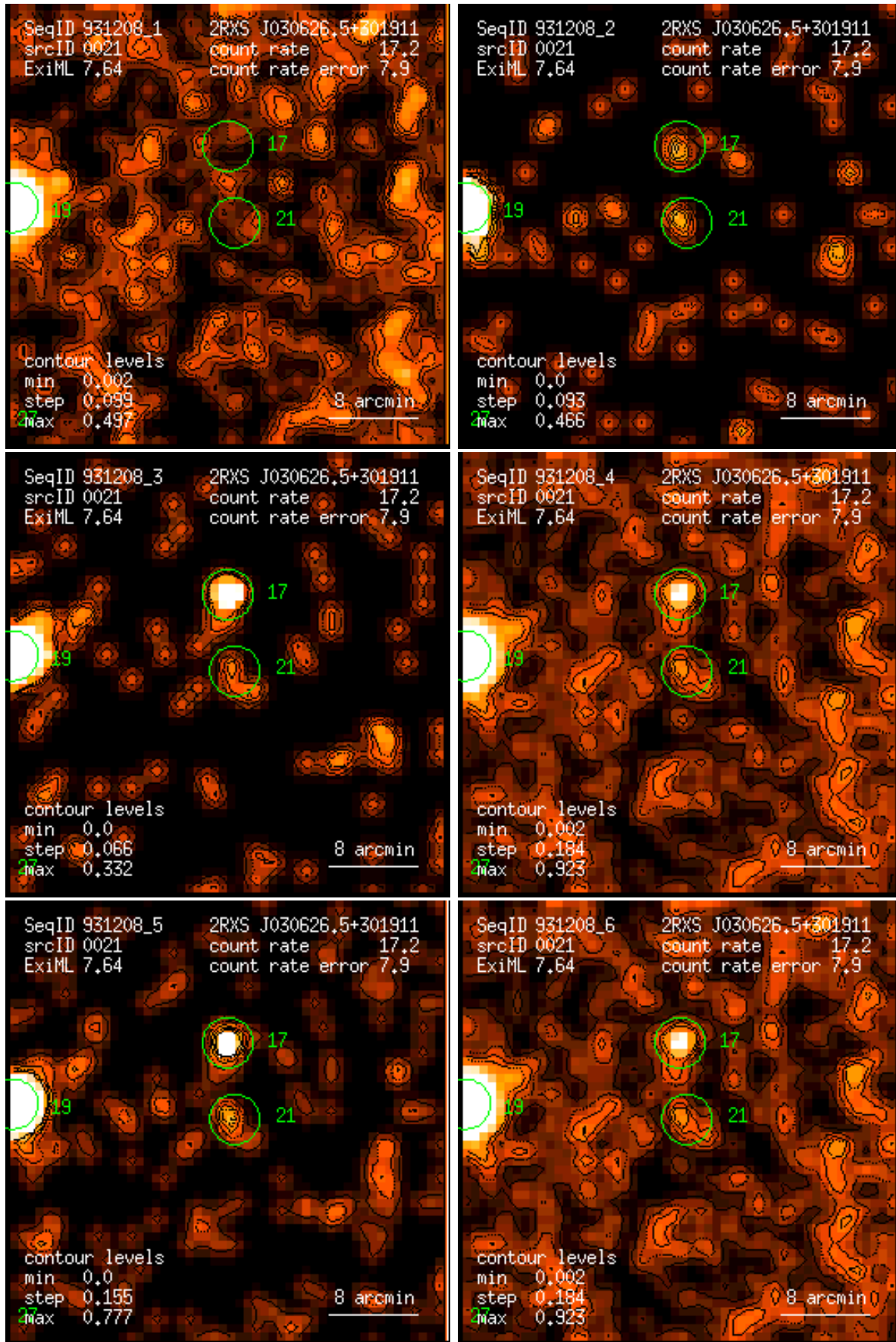
Figure 21: RASS 931208: detection 0021: band rate images, Gaussian filter: (1) PSPC channels 11 – 41, (2) 52 – 90, (3) 91 – 201, (4) 11 – 235, (5) 52 – 201, (6) 11 – 201. Broad band rates in counts/ks. Band rate contour levels in counts/ks/arcmin 2 .
