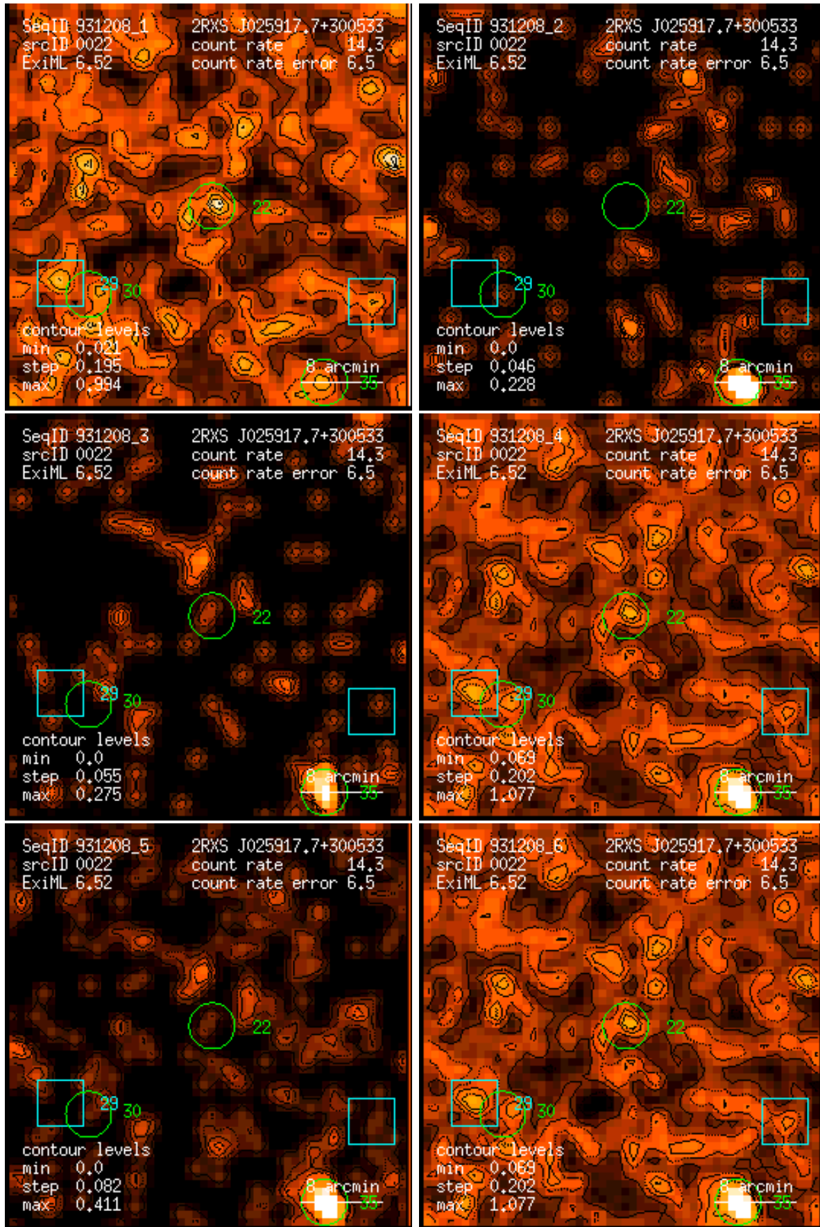
Figure 22: RASS 931208: detection 0022: band rate images, Gaussian filter: (1) PSPC channels 11 – 41, (2) 52 – 90, (3) 91 – 201, (4) 11 – 235, (5) 52 – 201, (6) 11 – 201. Broad band rates in counts/ks. Band rate contour levels in counts/ks/arcmin 2 .
