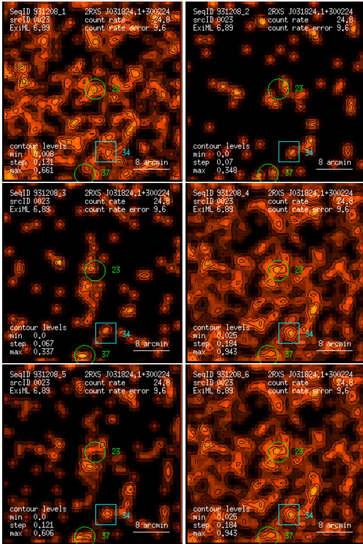
Figure 23: RASS 931208: detection 0023: band rate images, Gaussian filter: (1) PSPC channels 11 – 41, (2) 52 – 90, (3) 91 – 201, (4) 11 – 235, (5) 52 – 201, (6) 11 – 201. Broad band rates in counts/ks. Band rate contour levels in counts/ks/arcmin 2 .
