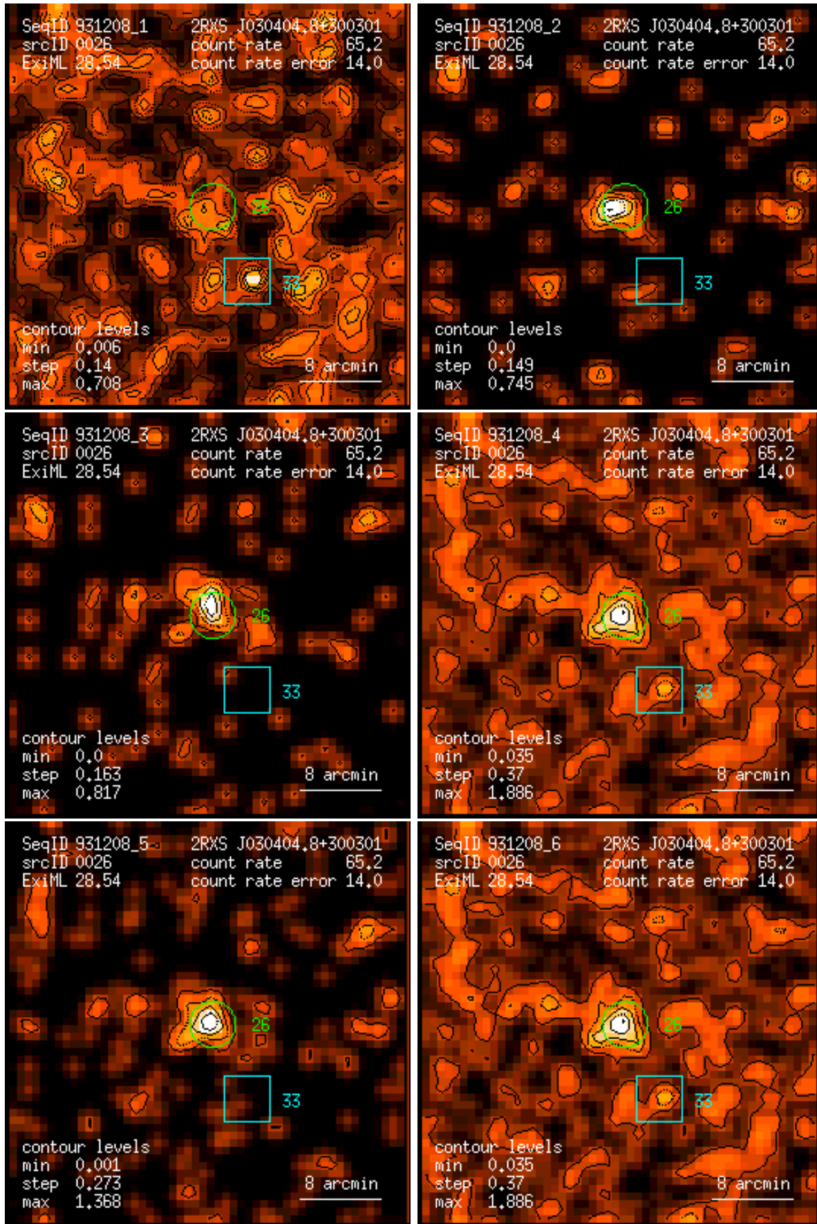
Figure 26: RASS 931208: detection 0026: band rate images, Gaussian filter: (1) PSPC channels 11 – 41, (2) 52 – 90, (3) 91 – 201, (4) 11 – 235, (5) 52 – 201, (6) 11 – 201. Broad band rates in counts/ks. Band rate contour levels in counts/ks/arcmin 2 .
