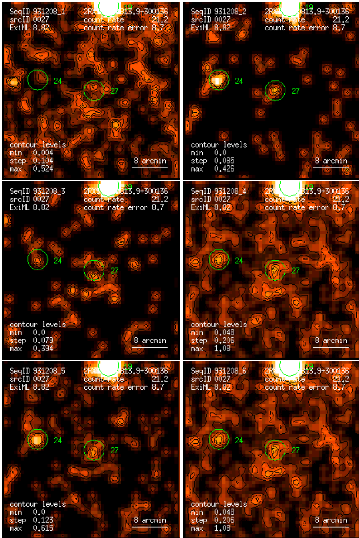
Figure 27: RASS 931208: detection 0027: band rate images, Gaussian filter: (1) PSPC channels 11 – 41, (2) 52 – 90, (3) 91 – 201, (4) 11 – 235, (5) 52 – 201, (6) 11 – 201. Broad band rates in counts/ks. Band rate contour levels in counts/ks/arcmin 2 .
