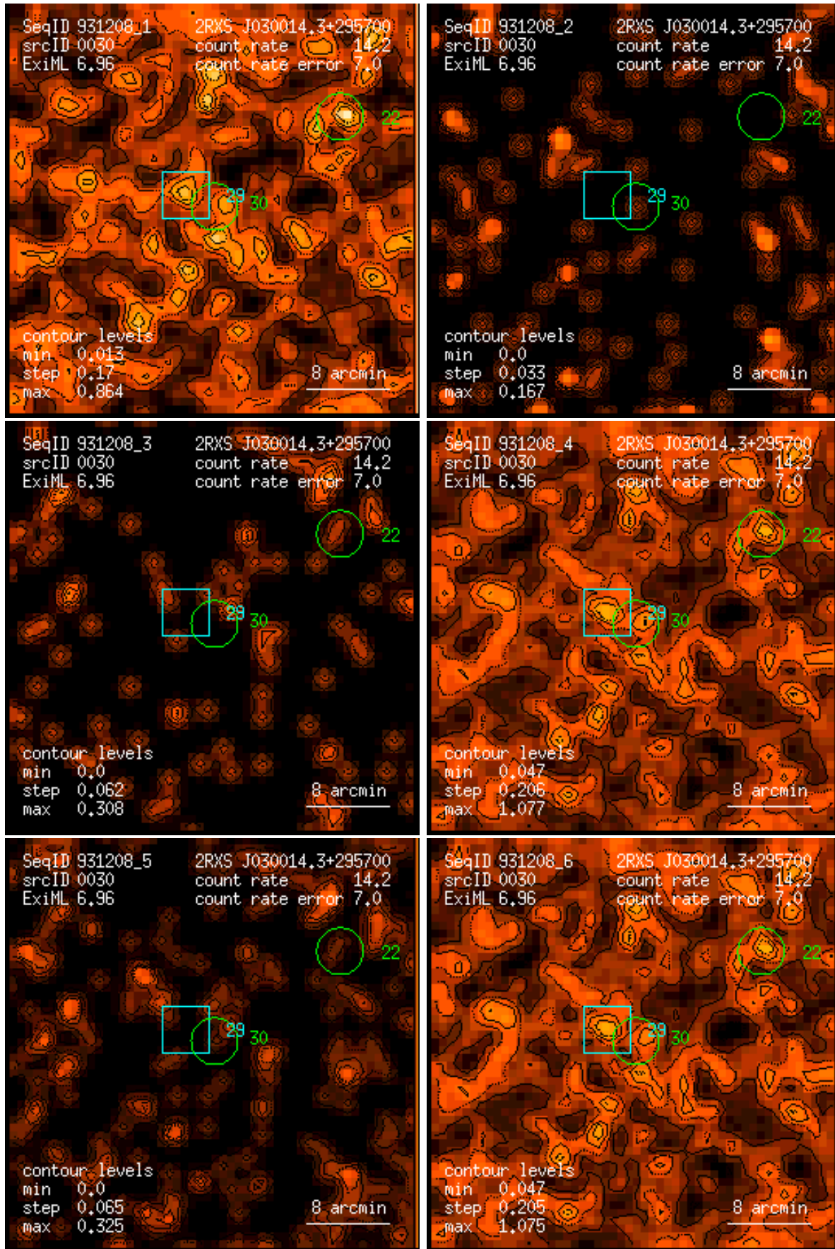
Figure 30: RASS 931208: detection 0030: band rate images, Gaussian filter: (1) PSPC channels 11 – 41, (2) 52 – 90, (3) 91 – 201, (4) 11 – 235, (5) 52 – 201, (6) 11 – 201. Broad band rates in counts/ks. Band rate contour levels in counts/ks/arcmin 2 .
