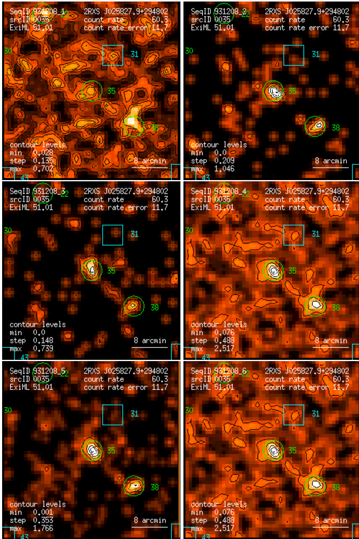
Figure 35: RASS 931208: detection 0035: band rate images, Gaussian filter: (1) PSPC channels 11 – 41, (2) 52 – 90, (3) 91 – 201, (4) 11 – 235, (5) 52 – 201, (6) 11 – 201. Broad band rates in counts/ks. Band rate contour levels in counts/ks/arcmin 2 .
