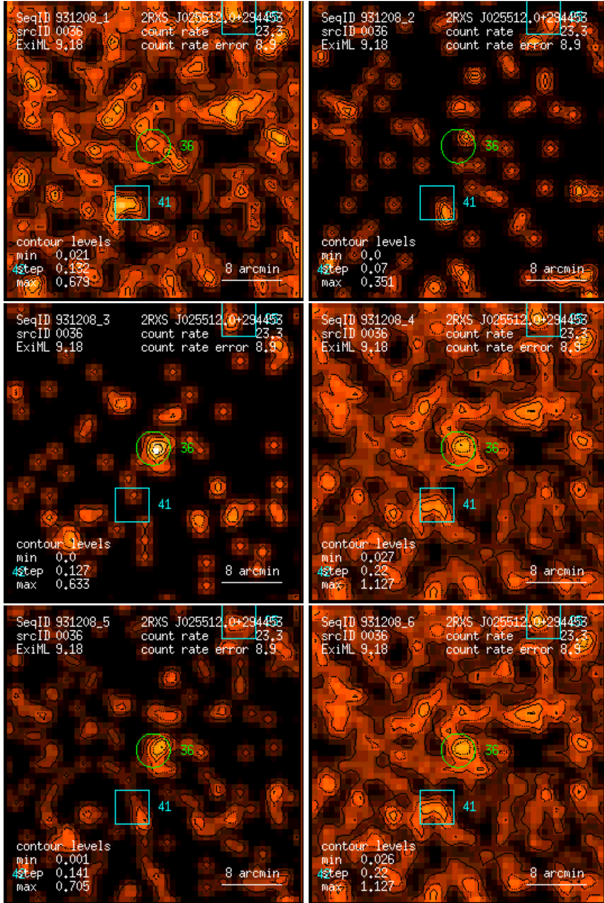
Figure 36: RASS 931208: detection 0036: band rate images, Gaussian filter: (1) PSPC channels 11 – 41, (2) 52 – 90, (3) 91 – 201, (4) 11 – 235, (5) 52 – 201, (6) 11 – 201. Broad band rates in counts/ks. Band rate contour levels in counts/ks/arcmin 2 .
