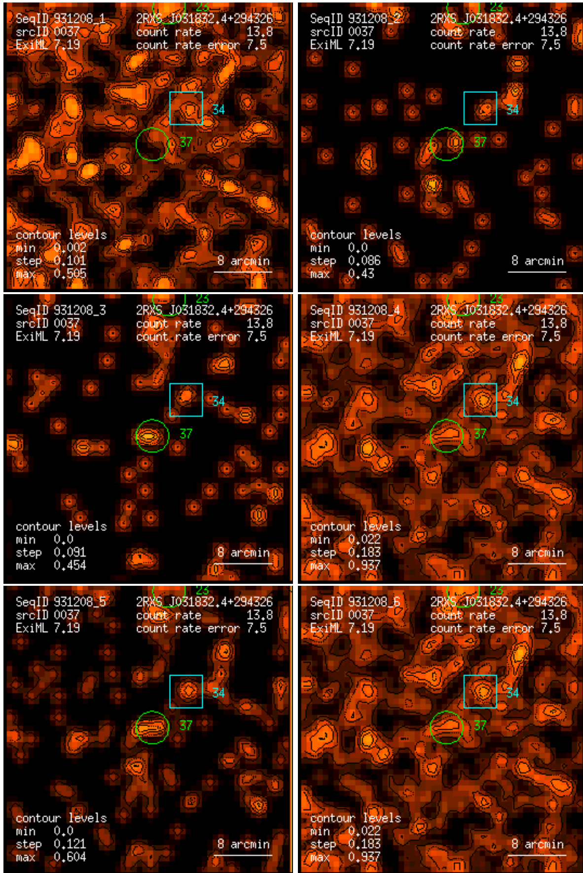
Figure 37: RASS 931208: detection 0037: band rate images, Gaussian filter: (1) PSPC channels 11 – 41, (2) 52 – 90, (3) 91 – 201, (4) 11 – 235, (5) 52 – 201, (6) 11 – 201. Broad band rates in counts/ks. Band rate contour levels in counts/ks/arcmin 2 .
