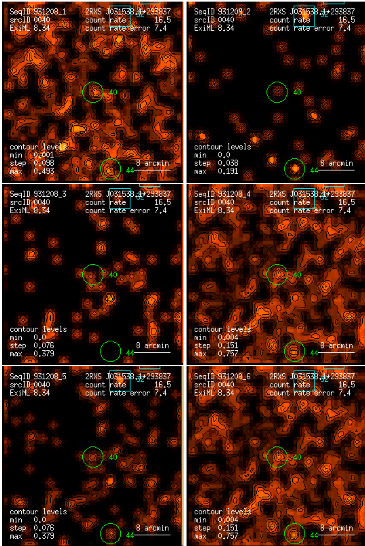
Figure 40: RASS 931208: detection 0040: band rate images, Gaussian filter: (1) PSPC channels 11 – 41, (2) 52 – 90, (3) 91 – 201, (4) 11 – 235, (5) 52 – 201, (6) 11 – 201. Broad band rates in counts/ks. Band rate contour levels in counts/ks/arcmin 2 .
