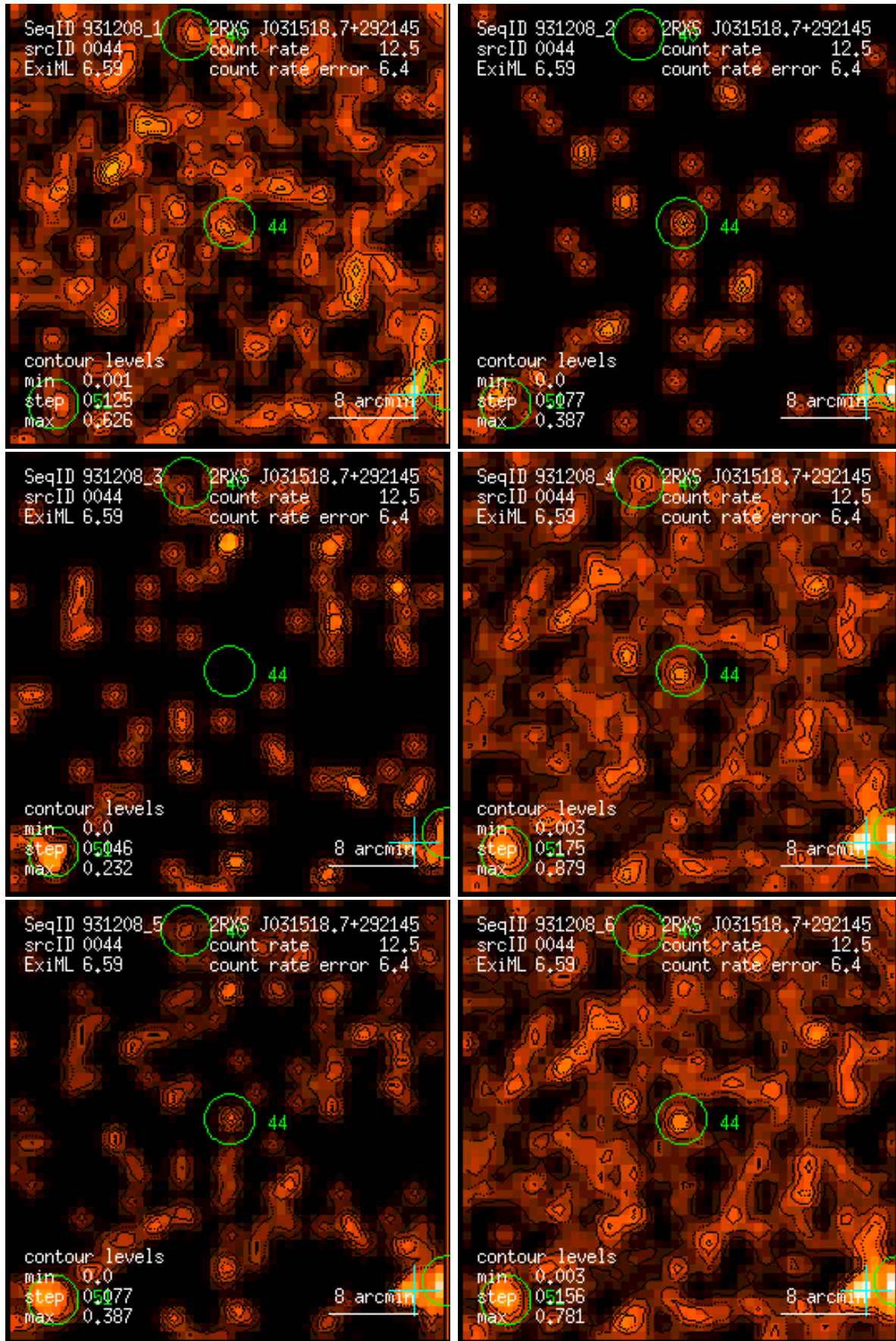
Figure 44: RASS 931208: detection 0044: band rate images, Gaussian filter: (1) PSPC channels 11 – 41, (2) 52 – 90, (3) 91 – 201, (4) 11 – 235, (5) 52 – 201, (6) 11 – 201. Broad band rates in counts/ks. Band rate contour levels in counts/ks/arcmin 2 .
