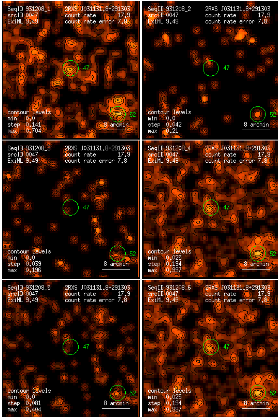
Figure 47: RASS 931208: detection 0047: band rate images, Gaussian filter: (1) PSPC channels 11 – 41, (2) 52 – 90, (3) 91 – 201, (4) 11 – 235, (5) 52 – 201, (6) 11 – 201. Broad band rates in counts/ks. Band rate contour levels in counts/ks/arcmin 2 .
