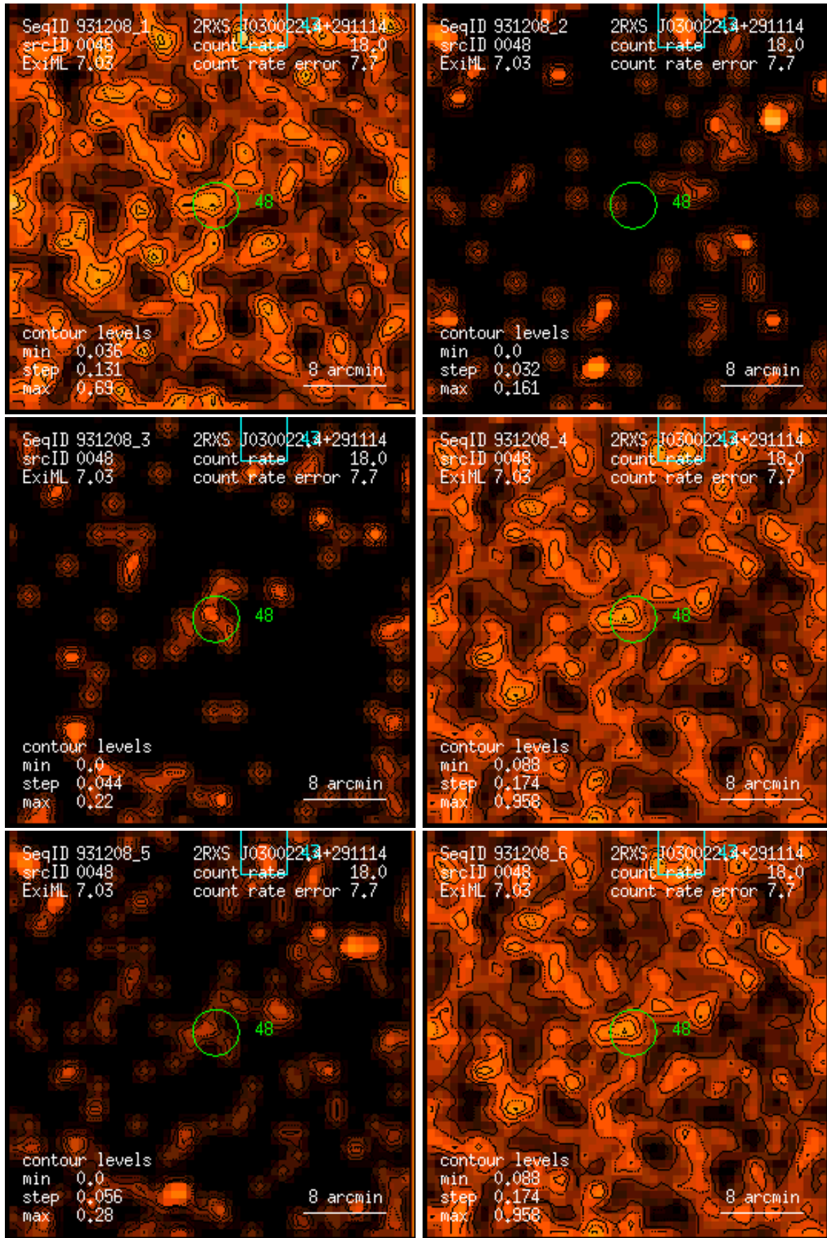
Figure 48: RASS 931208: detection 0048: band rate images, Gaussian filter: (1) PSPC channels 11 – 41, (2) 52 – 90, (3) 91 – 201, (4) 11 – 235, (5) 52 – 201, (6) 11 – 201. Broad band rates in counts/ks. Band rate contour levels in counts/ks/arcmin 2 .
