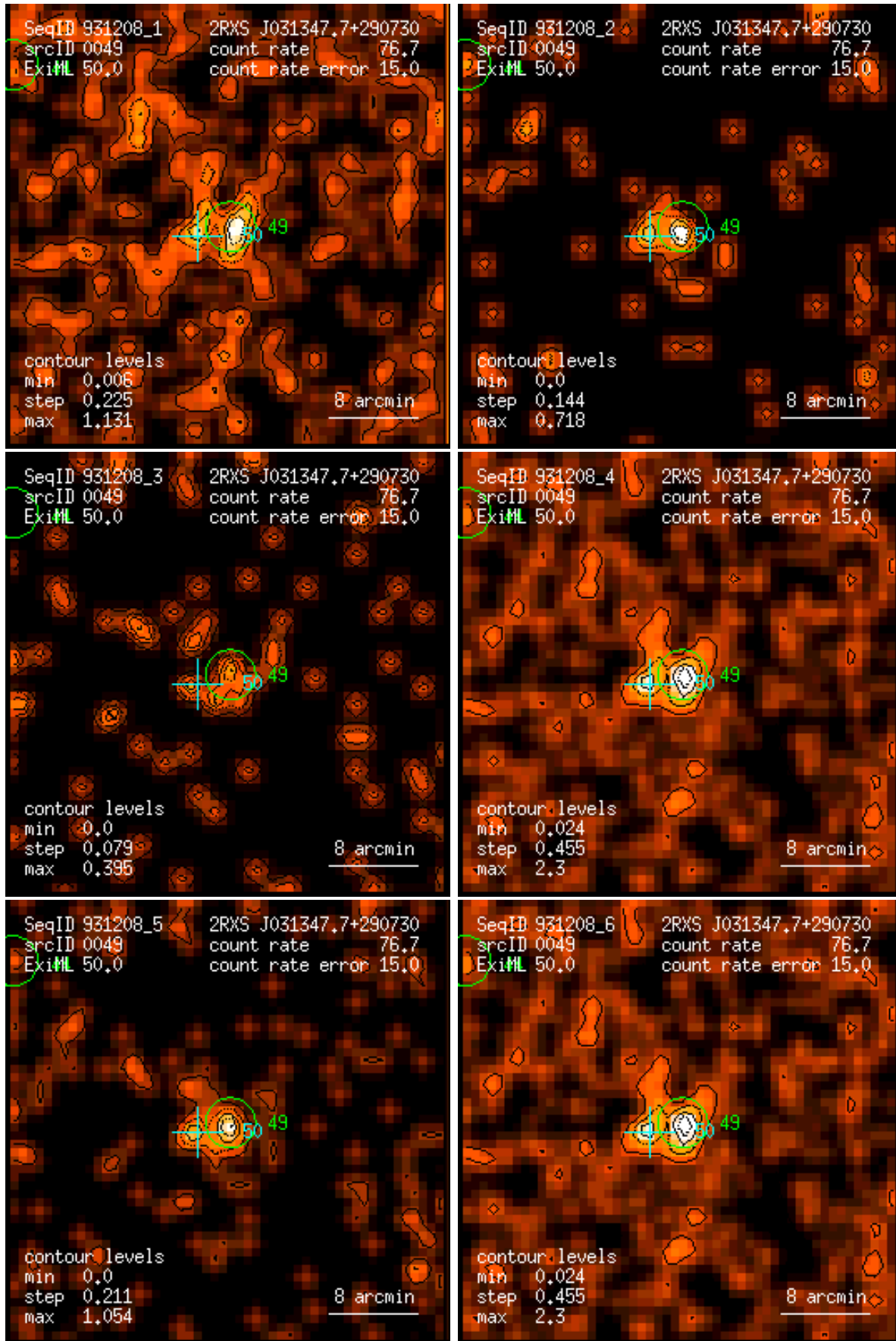
Figure 49: RASS 931208: detection 0049: band rate images, Gaussian filter: (1) PSPC channels 11 – 41, (2) 52 – 90, (3) 91 – 201, (4) 11 – 235, (5) 52 – 201, (6) 11 – 201. Broad band rates in counts/ks. Band rate contour levels in counts/ks/arcmin 2 .
