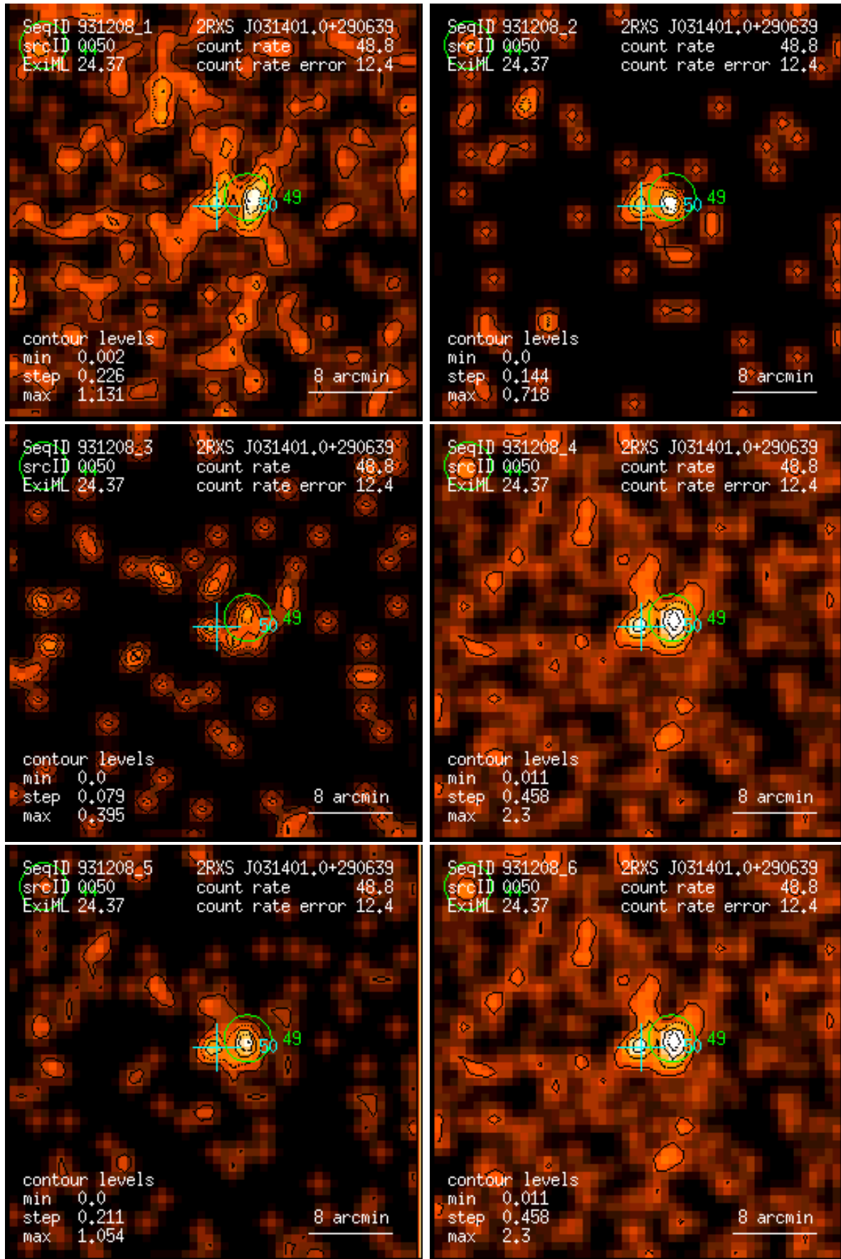
Figure 50: RASS 931208: detection 0050: band rate images, Gaussian filter: (1) PSPC channels 11 – 41, (2) 52 – 90, (3) 91 – 201, (4) 11 – 235, (5) 52 – 201, (6) 11 – 201. Broad band rates in counts/ks. Band rate contour levels in counts/ks/arcmin 2 .
